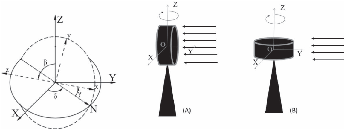
Figure 2. Left panel: laboratory, XYZ, and auxiliary, xyz, reference frames. Right panel: (A) particle in its initial position on the holder; (B) particle after a rotation of \beta = 90^\circ . Oxyz defines the laboratory reference frame. In both cases each orientation of the particle corresponds to a rotation around Z.
