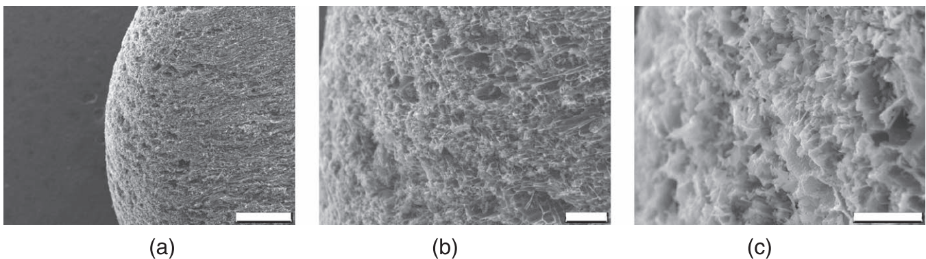
Figure 6. SEM images of the charcoal particle, border region. White bars denote (a) 500 \mu\text{m} , (b) 100 \mu\text{m} , and (c) 50 \mu\text{m} .
