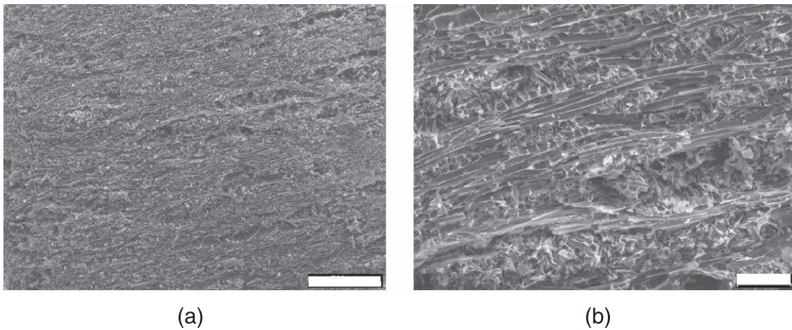
Figure 5. SEM images of the charcoal particle, central region. White bars denote (a) 500 \mu\text{m} and (b) 100 \mu\text{m} .
