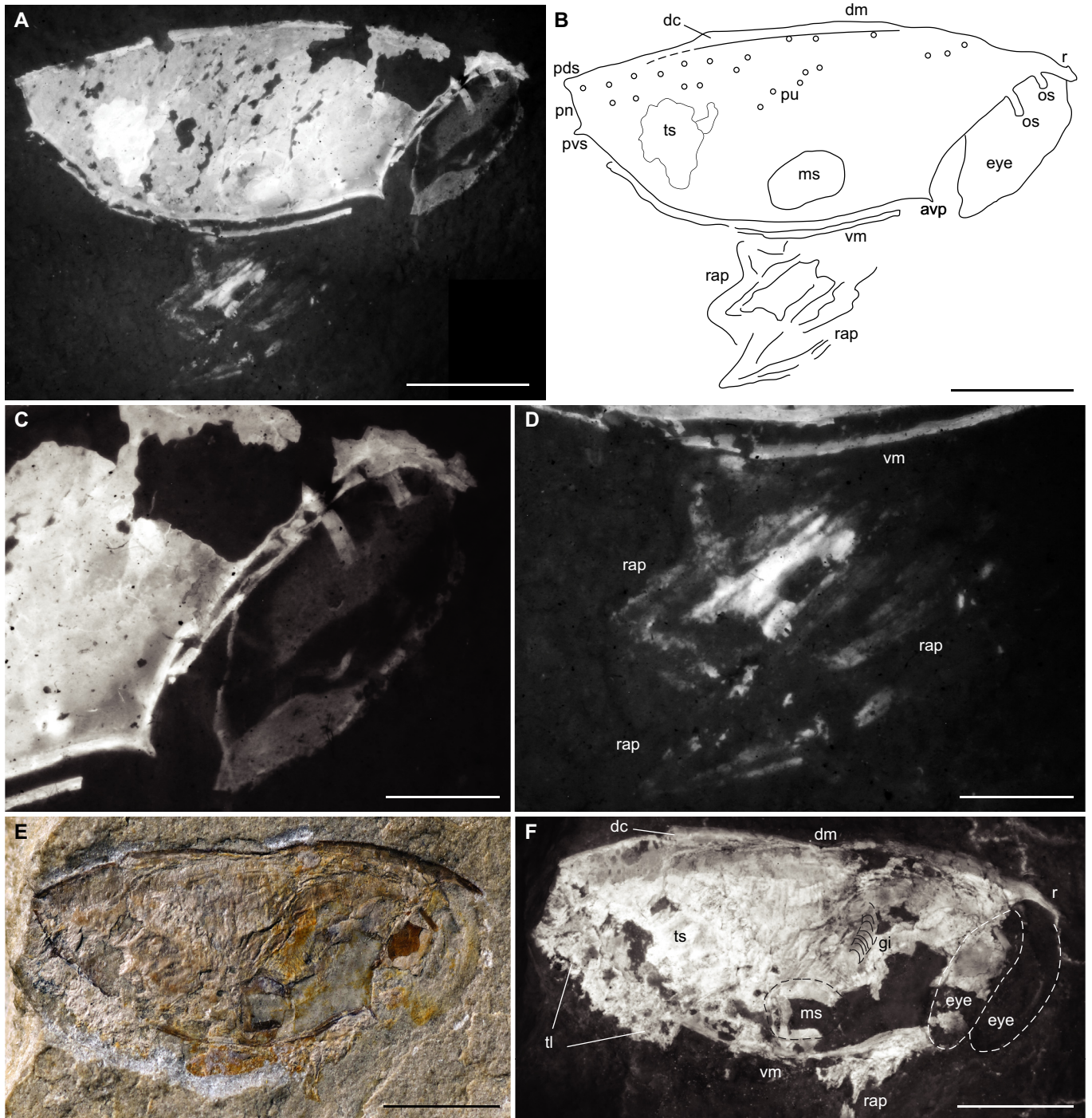
Fig. 7. Thylacocaris schrami Audo and Charbonnier nov. gen, nov. sp. from the Cenomanian of Hadjoula, Lebanon. A–D. Paratype MNHN.F. A57235, right lateral view, green-orange light desaturated, subcomplete specimen showing carapace, eye, and prominent anterior appendages (A), interpretative line drawing (B), close-up of optical notch with well-preserved eye, and two optic spines (C), close-up of anterior appendages (D). E–F. Paratype MSNM i25125, carapace, eyes and fragments of anterior appendages, natural light (E), green-orange light desaturated (F). Abbreviations: avp = antero-ventral process, dc = dorsal carina, dm = dorsal margin, gi = lamellate gills, ms = muscle scar, os = optical spine, pn = posterior notch, pu = punctuation, pds = postero-dorsal spine, pvs = postero-ventral spine, r = rostrum, rap = prominent anterior appendages, tl = paddle-like limbs or trunk limbs, ts = trunk somites, vm = ventral margin. Scale bars: 5 mm (A, B, E, F) and 2 mm (D). Line drawing: S. Charbonnier. Photographs: J. Haug (A, C, D, F) and L. Cazes (E).
