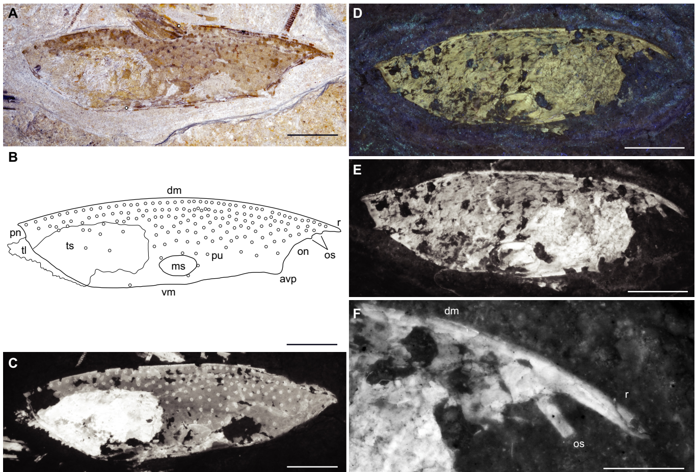
Fig. 8. Thylacocaris schrami Audou and Charbonnier nov. gen, nov. sp. from the Cenomanian of Hadjoula, Lebanon. A–C. Paratype MNHN.F. A57244, carapace, right lateral view, natural light (A), line drawing (B), green-orange light desaturated, before preparation (C). D–F. Paratype MSNM i24785, carapace, right lateral view, UV light (D), green-orange light desaturated (E), close-up of rostrum (F). Abbreviations: avp = antero-ventral process, dm = dorsal margin, ms = muscle scar, on = optical notch, os = optical spine, pn = posterior notch, pu = punctuation, r = rostrum, tl = paddle-like limbs or trunk limbs, ts = trunk somites, vm = ventral margin. Scale bars: 5 mm (A–E) and 2 mm (F). Line drawing: M. Lasseron. Photographs: D. Audou (A), J. Haug (C, E, F) and L. Cazes (D).
