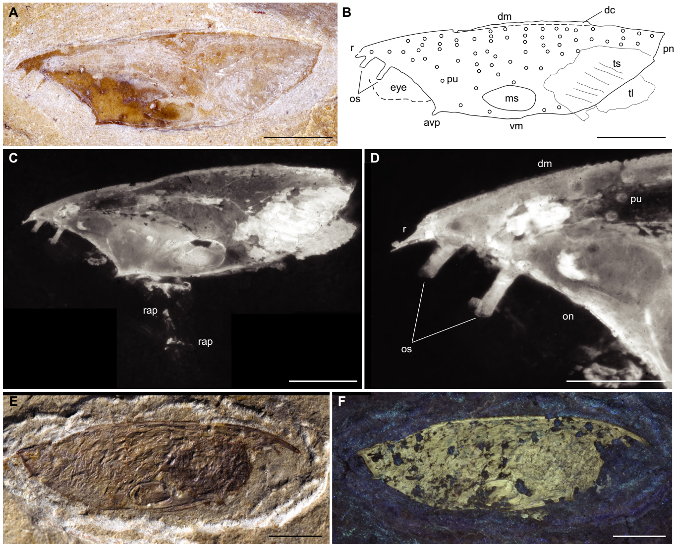
Fig. 6. Thylacocaris schrami Audo and Charbonnier nov. gen, nov. sp. from the Cenomanian of Hadjoula, Lebanon. A–D. Holotype MNHN.F. A57240, left lateral view, cross-polarized light (A), line-drawing of carapace, and soft-parts (B), carapace and fragments of anterior prehensile appendages, green-orange fluorescence desaturated (C), close-up of optical notch showing broken rostrum and two optical spines, green-orange fluorescence desaturated (D). E–F. Paratype MSNM i24785, carapace, right lateral view, natural light (E), UV light (F). Abbreviations: avp = antero-ventral process, dc = dorsal carina, dm = dorsal margin, ms = muscle scar, on = optical notch, os = optical spine, pn = posterior notch, pu = punctuation, rap = prominent anterior appendages, tl = paddle-like limbs or trunk limbs, ts = trunk somites, vm = ventral margin. Scale bars: 5 mm (A–C, E, F) and 2 mm (D). Line drawing: S. Charbonnier. Photographs: D. Audo (A), J. Haug (C, D) and L. Cazes (E–F).
