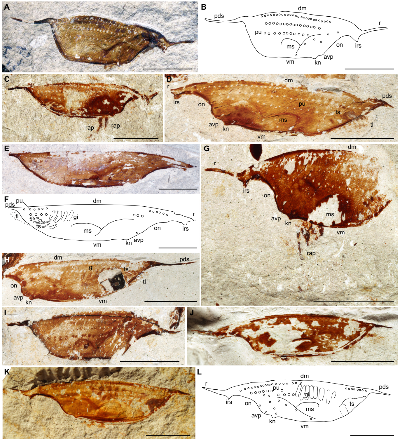
Fig. 10. Hamaticaris damesi (Roger, 1946), nov. gen., nov. comb. the Santonian of Sahel Alma, Lebanon. A–B. Paralectotype MNHN.F.B18842, carapace, right lateral view (A) and interpretative line drawing (B). C. Lectotype MNHN.F.B18843, carapace, right lateral view, note the anterior prehensile appendages. D. Paralectotype MNHN.F.A30668, carapace, left lateral view. E–F. Paralectotype MNHN.F.A30652, carapace, right lateral view (E) and interpretative line drawing (F). G. Paralectotype MNHN.F.A30655, fragment of carapace, left lateral view. H. Paralectotype MNHN.F.A30669, carapace, left lateral view. I. Paralectotype MNHN.F.A30659, carapace, right lateral view, note the Y-shaped ridges. J. Paralectotype MNHN.F.A30672, carapace, left lateral view. K–L. Paralectotype MNHN.F.A30656, carapace, left lateral view (K) and interpretative line drawing (L). Abbreviations: avp = antero-ventral process, dm = dorsal margin, gi = gills, irs = infra-rostral spine, kn = knob, ms = muscle scar, on = optical notch, pu = punctuation, pds = postero-dorsal spine, r = rostrum, rap = prominent anterior appendages, ts = trunk somites, tl = paddle-like limbs or trunk limbs, vm = ventral margin. Scale bars: 5 mm. Line drawing: S. Charbonnier. Photographs all in cross-polarized light: J. Haug and G. Doitieu (K).
