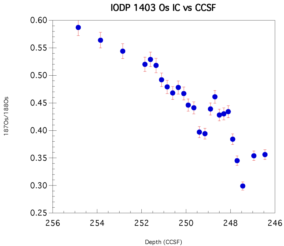
Fig. S20. Osmium isotope record from IODP Site U1403, with 95% confidence intervals.
