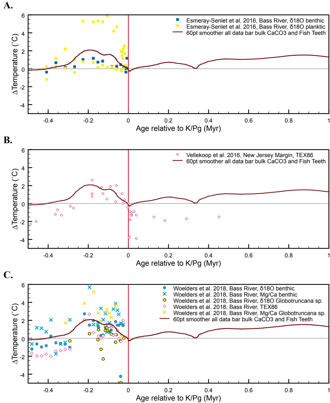
Fig. S8. Temperature records from Bass River (A) \delta^{18}\text{O} of foraminifera (132), (B) TEX 86 (144), and (C) mixed proxies (145), on unified age models and a common \delta^{18}\text{O} -temperature equation.
