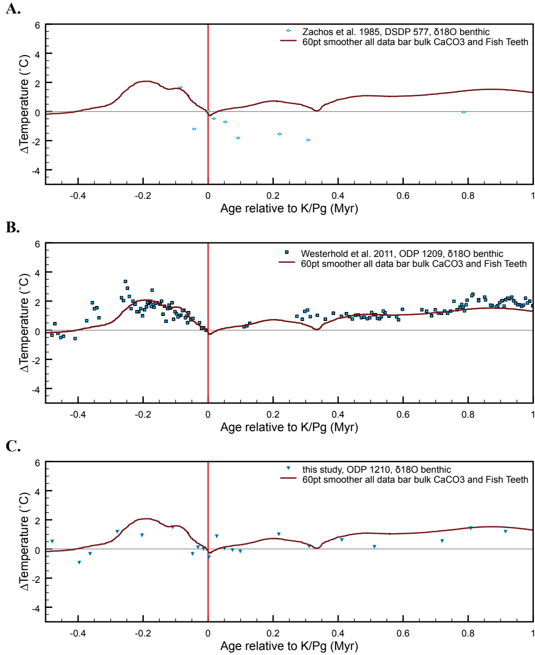
Fig. S3. Temperature records from Shatsky Rise sites: (A) DSDP Site 577 (90), (B) ODP Site 1209 (73), and (C) ODP Site 1210 ( this study ), on unified age models and a common \delta^{18} O-temperature equation.
