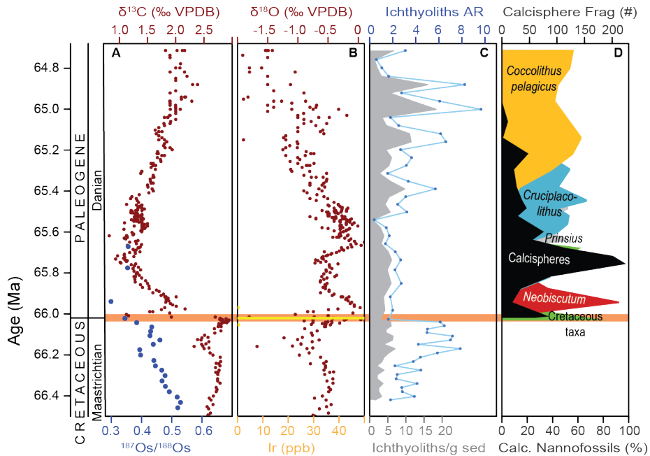
506 Figure 5. Late Cretaceous warming and early Paleocene record of environmental and 507 biotic change at IODP Site U1403, J-Anomaly Ridge, Newfoundland. A negative carbon 508 isotope anomaly (A) coincides with late Cretaceous warming in \delta^{18}\text{O} (B), and osmium isotope 509 evidence for volcanism (A) at IODP Site U1403. The collapse in surface ocean \delta^{13}\text{C} values (A) 510 coincides with iridium anomaly (B), and step change in fish tooth accumulation (C). Earliest 511 Paleocene \delta^{18}\text{O} values of bulk carbonate appear to be strongly influenced by vital effects driven 512 by rapid turnover in the dominant calcareous nannofossil taxa (D) in sites globally (Figs. S18, 513 S34, S35). Data in Tables S12, S16, S17, S29.
