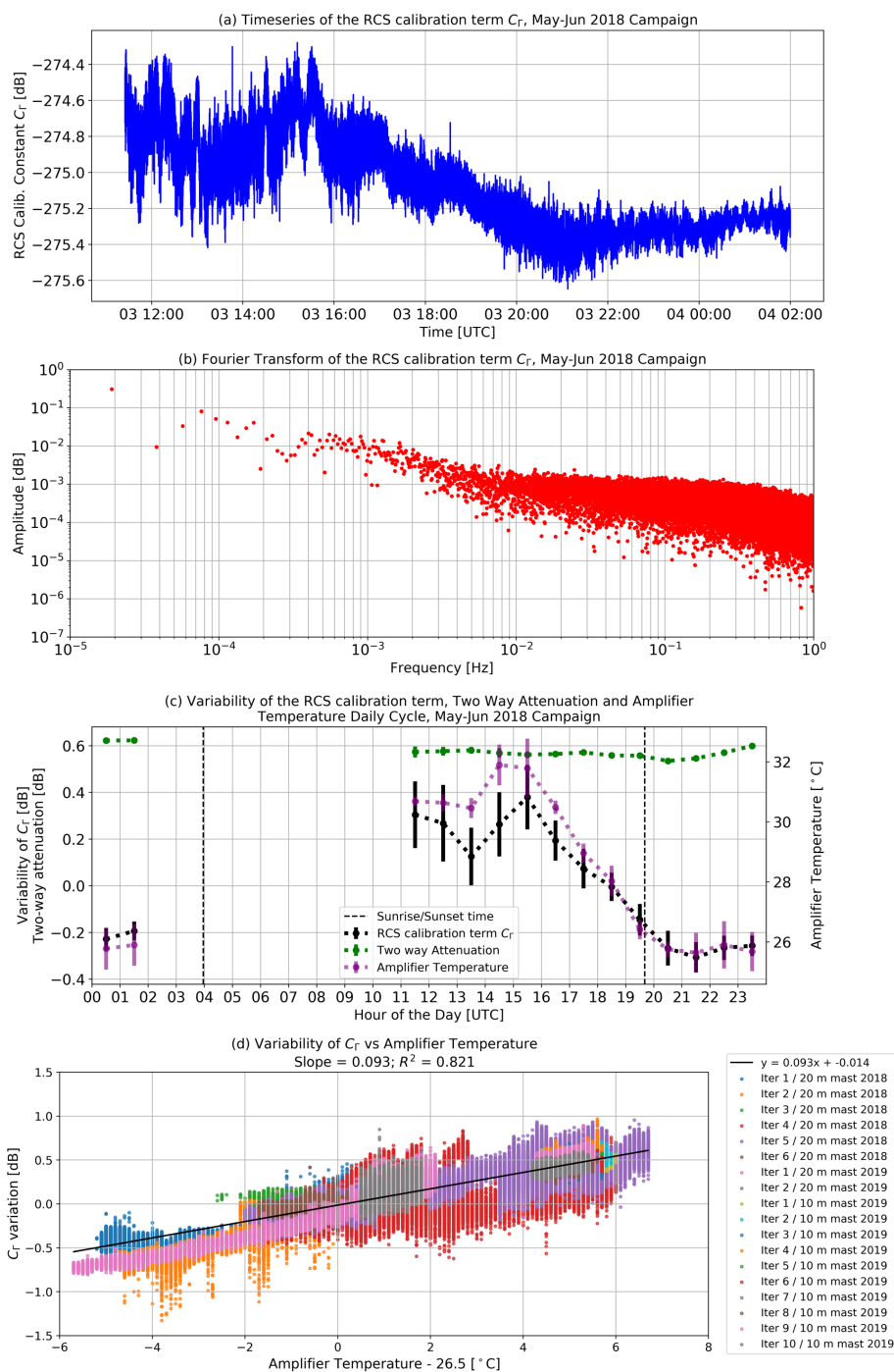
Figure 5. Study of calibration variability. Samples from iteration 5, 2018 Calibration Campaign. (a) Time series of the RCS Calibration term retrieval. (b) Fourier transform of the RCS Calibration term after subtracting the mean value. (c) Daily Cycle of calibration variability, amplifier temperature and two-way attenuation. Attenuation errorbars are too small to be seen with this scale. (d) Regression of the relative changes in the C_r(T) versus amplifier temperature, calculated using all samples from 2018 and 2019 campaigns.
