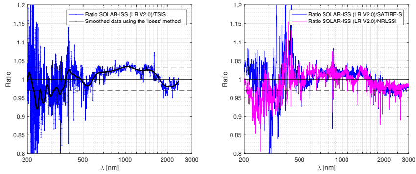
Figure 6. Left: Ratio to SOLAR-ISS (V2.0) for TSIS. Right: Ratio to SOLAR-ISS (V2.0) for SATIRE-S and NRL-SSI. We also observe that the correlations between the models (SATIRE-S and NRL-SSI) and TSIS are excellent.
