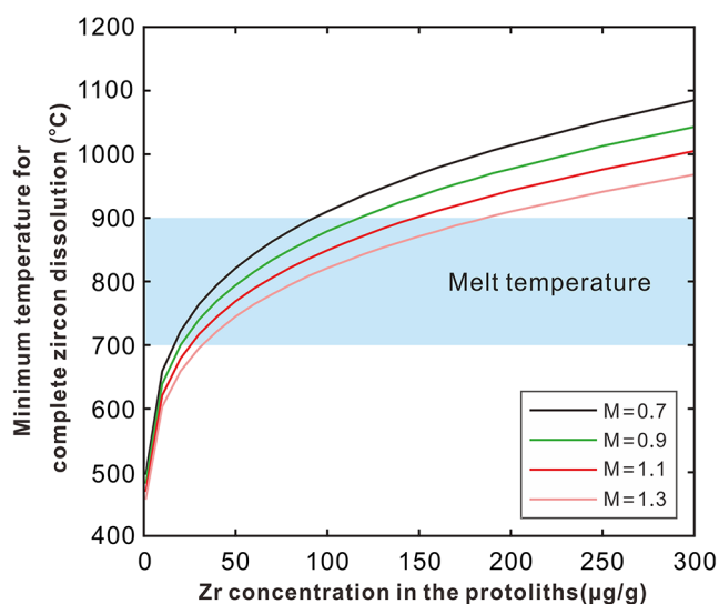
Figure 4 Calculated minimum melt temperature for zircon dissolution as a function of Zr concentration in the protoliths and M value (cation ratio). SPG have M values > 1.1 while I-type granites typically have M values < 1.0. Melt Zr concentration at zircon saturation using the zircon saturation model of Boehnke et al. (2013).
