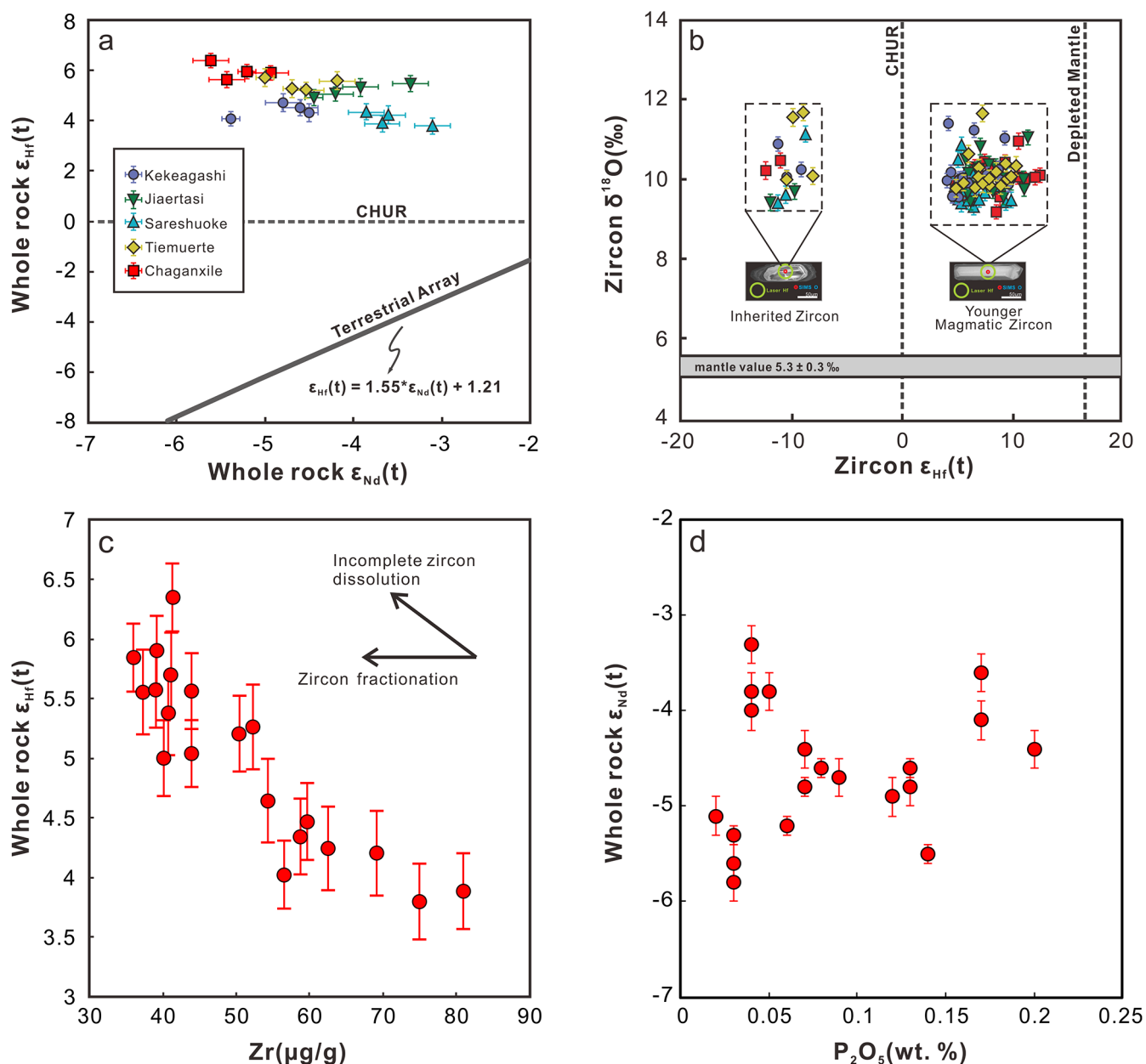
Figure 1 (a) \epsilon_{Hf}(t) versus \epsilon_{Nd}(t) for SPG in the Chinese Altai calculated based on U-Pb ages of the various plutons. Terrestrial array equations are from Vervoort et al. (2011). (b) Zircon \epsilon_{Hf}(t) versus zircon \delta^{18}O for SPG in the Chinese Altai. Mantle values after Valley et al. (1998). Inherited zircons show \epsilon_{Hf}(t) and \delta^{18}O values, indicating a metasedimentary source. Younger magmatic zircons show positive \epsilon_{Hf}(t) values and similarly high \delta^{18}O values, CHUR-chondritic uniform reservoir. (c) \epsilon_{Hf}(t) versus Zr ( \mu\text{g/g} ). (d) \epsilon_{Nd}(t) versus P_2O_5 (wt. %). Uncertainties of all isotope measurements are internal 2\sigma .
