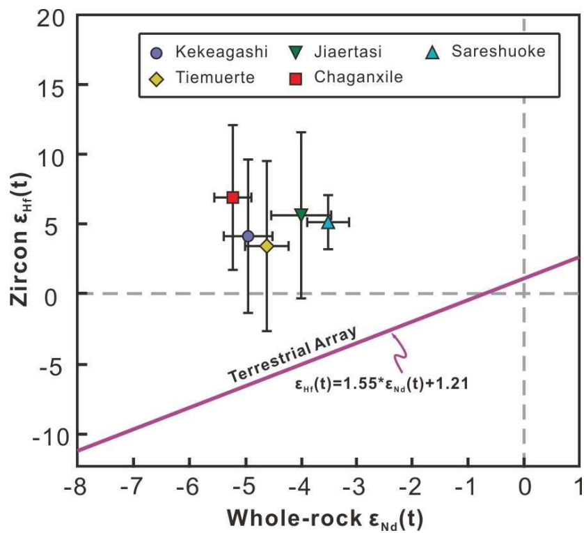
Figure S-6 Crossplot of zircon \epsilon_{Hf}(t) versus whole-rock \epsilon_{Nd}(t) .
