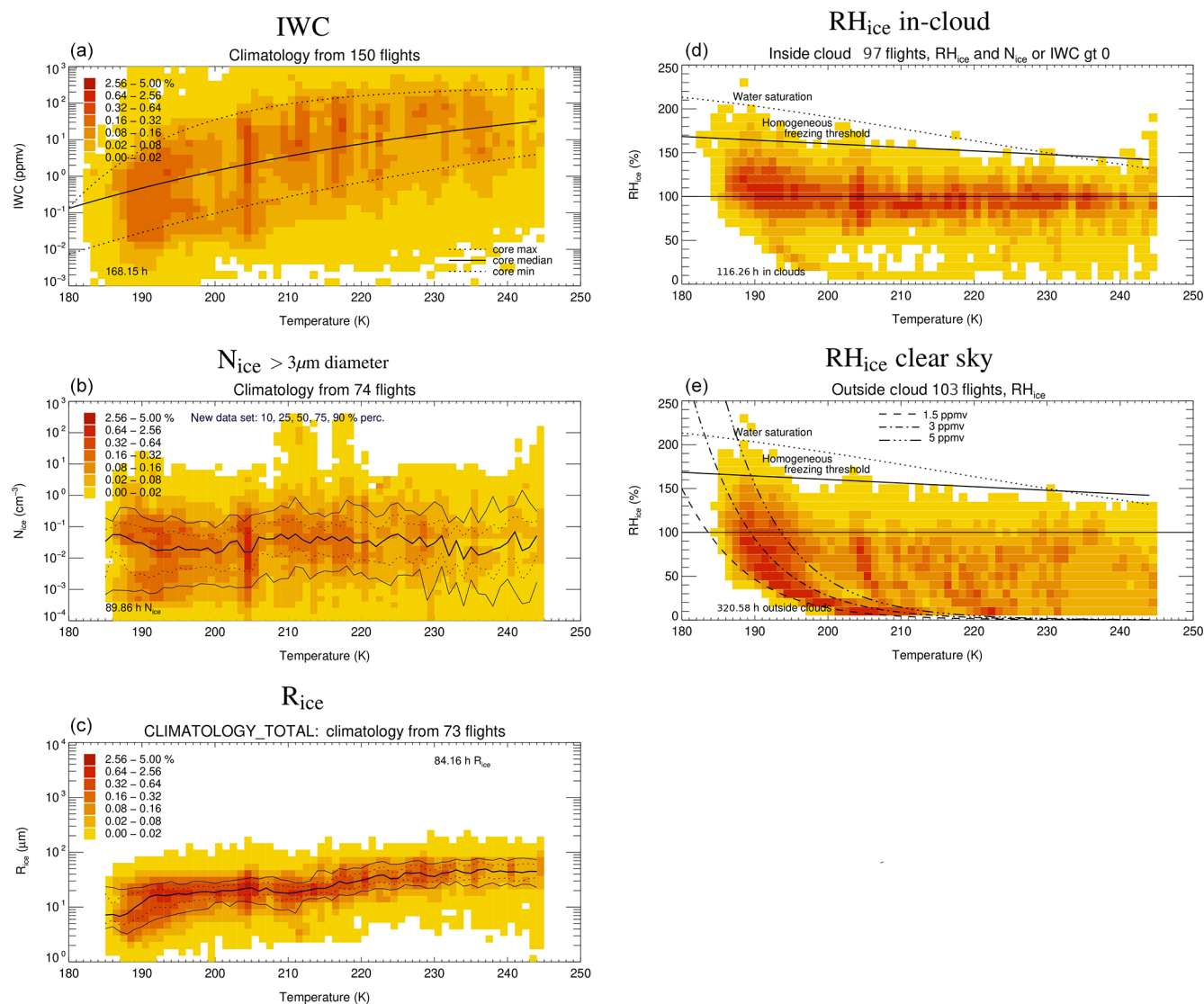
Figure A1. Data coverage of the Cirrus Guide II in situ database: IWC, N_{ice} , R_{ice} , and in-cloud and clear-sky RH_{ice} frequencies of occurrence as a function of temperature.
