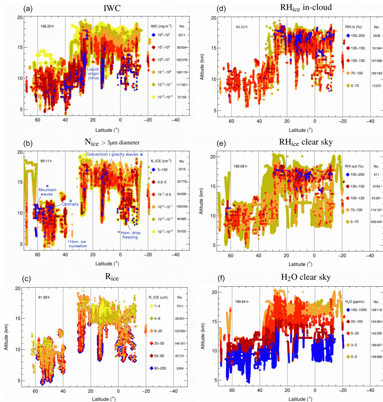
Figure 3. Cirrus cloud distribution with latitude and altitude of (left column, panels a–c ) ice water content (IWC, a ), ice crystal number ( N_{ice} , size > 3 μm diameter, b ), and mean mass radius ( R_{ice} , calculated from IWC/N_{ice} , c ). (Right column, panels d–f ) In-cloud and clear-sky relative humidity with respect to ice ( RH_{ice} , d , e ) and clear-sky water vapor volume mixing ratio ( H_2O , f ). The field campaigns are listed in Table A1, and data evaluation methods and detection ranges of the parameters are described in Appendix A. The color codes range from yellow to blue with increasing amount of the respective parameter; for R_{ice} , the color code is reversed to indicate that high and low N_{ice} values belong to small and large R_{ice} ; note that the data points are plotted in the order of the colors from yellow to blue; frequencies of occurrence of the parameters can be seen in Fig. 7.
