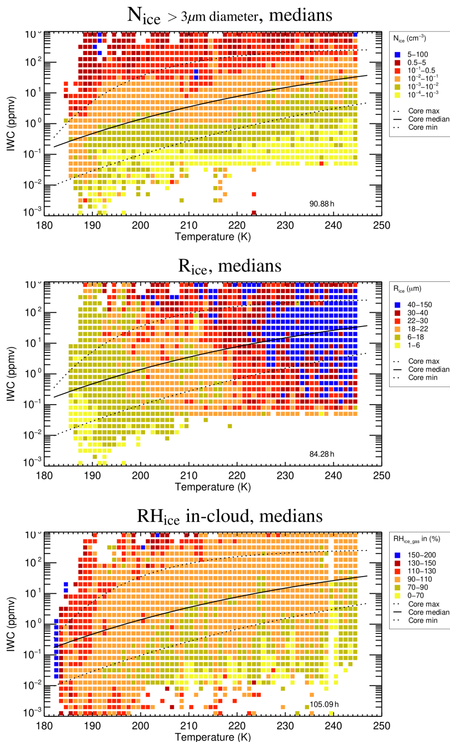
Figure 6. Median N_{\text{ice}} , R_{\text{ice}} , and RH_{\text{ice}} in intervals in the IWC– T parameter space (five IWC intervals per order of magnitude, 1 K temperature intervals). The color codes of N_{\text{ice}} and RH_{\text{ice}} range from yellow to blue with increasing amount of the respective parameter; for R_{\text{ice}} , the color code is reversed to indicate that high and low N_{\text{ice}} values belong to small and large R_{\text{ice}} . Black solid and dotted lines: median, min, and max IWC of the core IWC band of Schiller et al. (2008). The variability of the parameters (25th, 50th (median), and 75th percentiles) is shown in Figs. S1–S3 of the Supplement.
