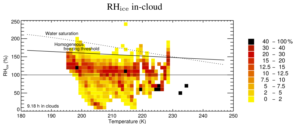
Figure A4. Example of biased \text{H}_2\text{O} measurements, visible in the in-cloud \text{RH}_{\text{ice}} frequencies: inside of cirrus clouds, at temperatures \gtrsim 200 \text{ K} , the frequencies should center around saturation (see Fig. 7d).
