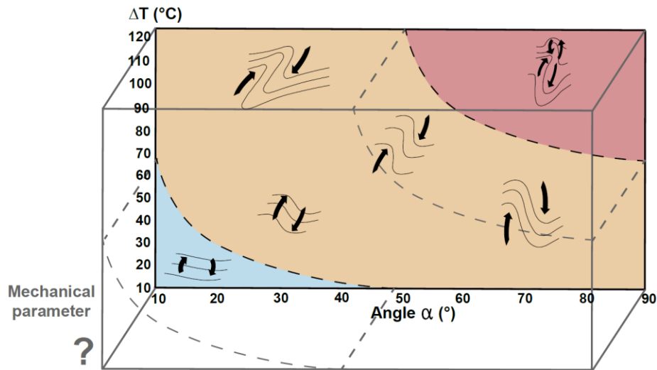
Figure 8 : Diagram of 2D convective regimes for the theoretical fault. The third variable, which may be used for 3D THM experiments, has yet to be determined.
