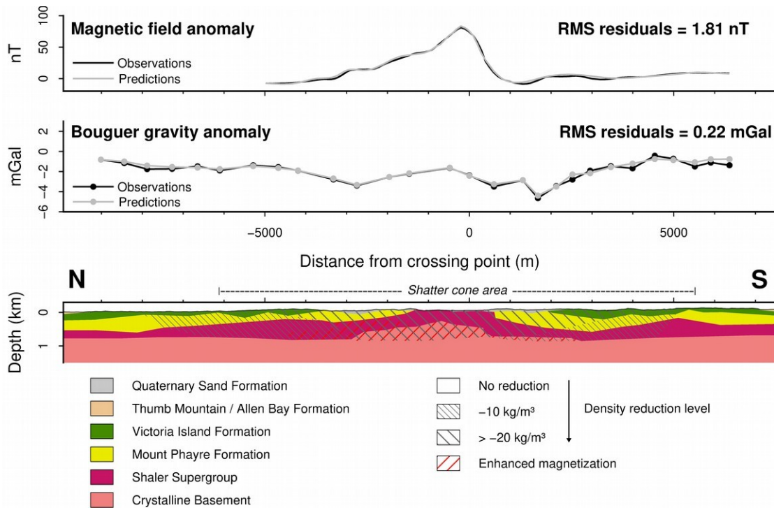
Fig. 6. N-S profile modeling of the Tunnunik impact structure constrained by magnetic and gravity data, as well as by laboratory measurements on samples. Top: comparison of observed (black) and predicted (gray) magnetic and gravity anomaly data. Location of the gravity measurements are shown by the solid points. Bottom: corresponding forward numerical model of the crust over the center of the Tunnunik impact structure. The physical parameters of each layer are shown in Table 1. Fracturing and brecciation (symbolized by gray hatching) decrease the bulk density values of all geological layers from the outer parts of the crater to the center. Topographic variations are from the global digital elevation model version 2 (GDEM2) of ASTER (NASA-METI). No vertical exaggeration.
