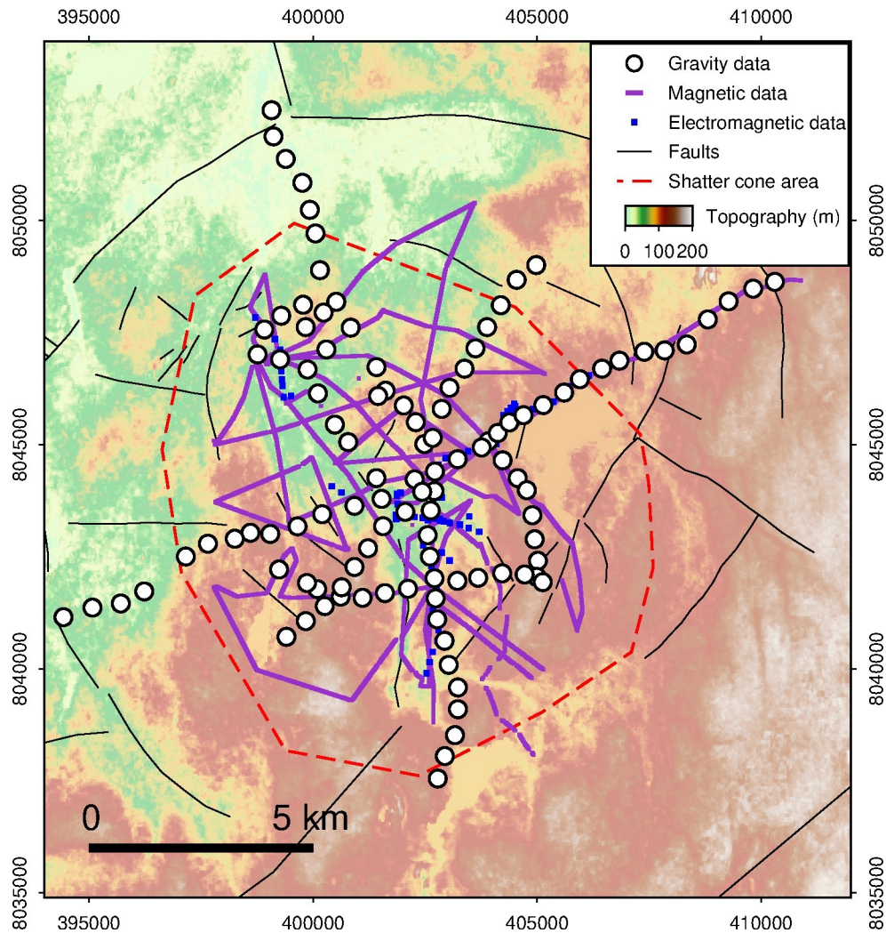
Fig. 2. Geophysical measurements performed at Tunnunik. Background corresponds to a digital elevation model version 2 (GDEM2) from ASTER (NASA-METI). Same coordinate system as for Fig. 1.
