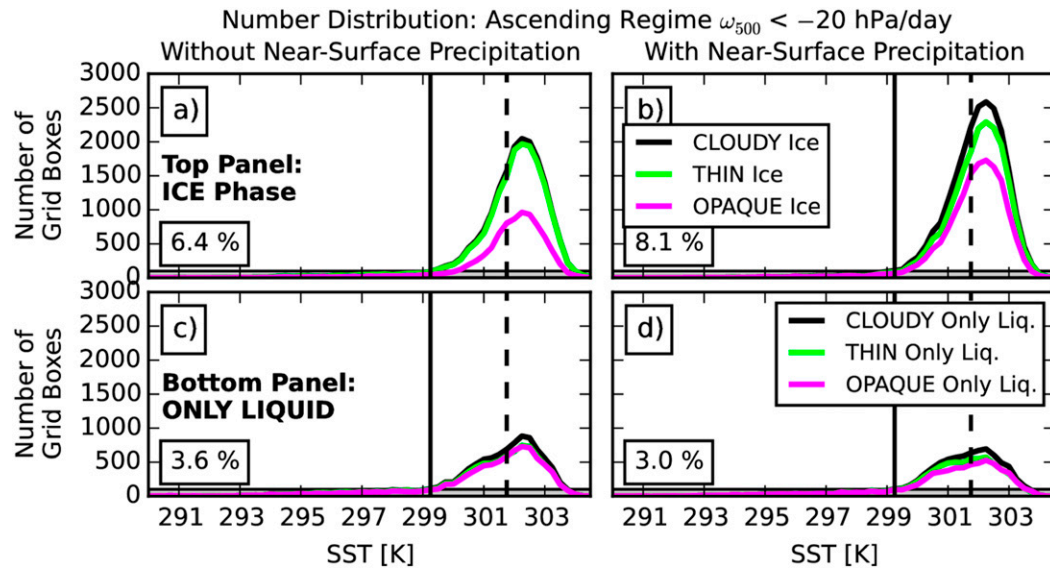
FIG. 7. Gridbox number distributions with SST for the ascending regime: \omega_{500} < -20 hPa day ^{-1} . Occurrence of grid boxes containing (a) ice clouds but no near-surface precipitation, (b) ice clouds and near-surface precipitation, (c) only liquid clouds but no near-surface precipitation, and (d) only liquid clouds and near-surface precipitation. Vertical lines are for the same SST thresholds as identified in Fig. 3.
