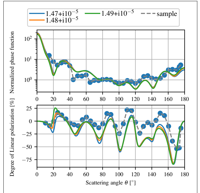
Fig. 2. Comparison of normalized phase function (at 90^\circ ) and the degree of linear polarization for levitating particles (measurements, bullets) and small clusters of spherical particles with varying refractive indices (computations, solid lines). Empirical phase function and degree of polarization are also depicted (dashed line).
