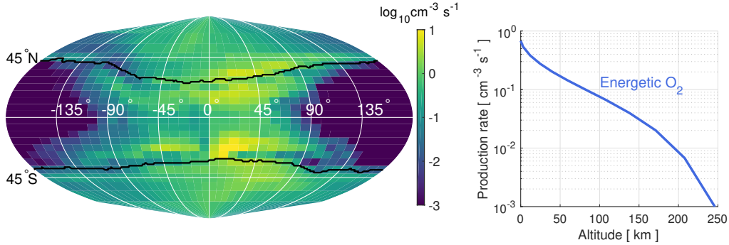
Figure A.8: Left panel: Map of O 2 production rate from charge-exchange with O 2 + at the surface. In the longitudinal direction, 0° and 90° correspond to the bisectors of, respectively, the leading and Jovian-facing hemispheres. The black curves show the OCFB lines obtained from the MHD model of Jia et al. (2009). The color scale is logarithmic. Right panel: Average (over latitude and longitude) production rate of O 2 from charge-exchange with O 2 + as a function of altitude.
