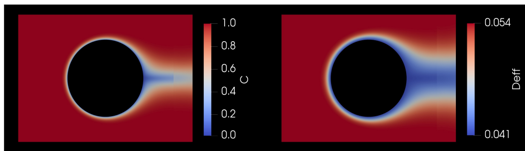
Fig. 7. Undersaturation ( C ) and diffusion ( D_{eff} ) fields around a cylindrical disk. The color scale indicates the variation in concentration (left) and effective diffusion coefficient Eq. (3) (right). The scale bar in the right panel indicates the ratio D_{eff}/\langle u \rangle (mm), where \langle u \rangle is the mean fluid velocity in the channel.
