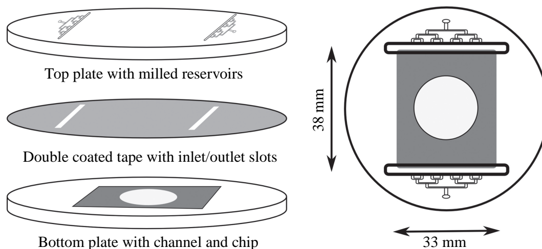
Fig. 1. Sketch of the microfluidic cell showing the three layer composition. The top polycarbonate plate has a network of microfluidic channels that deliver a uniform flow of liquid to the inlet reservoirs and a similar network at the outlet. The bottom plate is flat, apart from a shallow (0.5 mm) rectangular indentation where the gypsum disk is positioned. Fluid flows around the disk in the Hele-Shaw cell formed by the upper plate and the indented (gray) region in the bottom plate. An ultra-thin, double-coated tape is inserted between the two polycarbonate plates to seal them. The cell was modified from the original design in Osselin et al. (2016).
