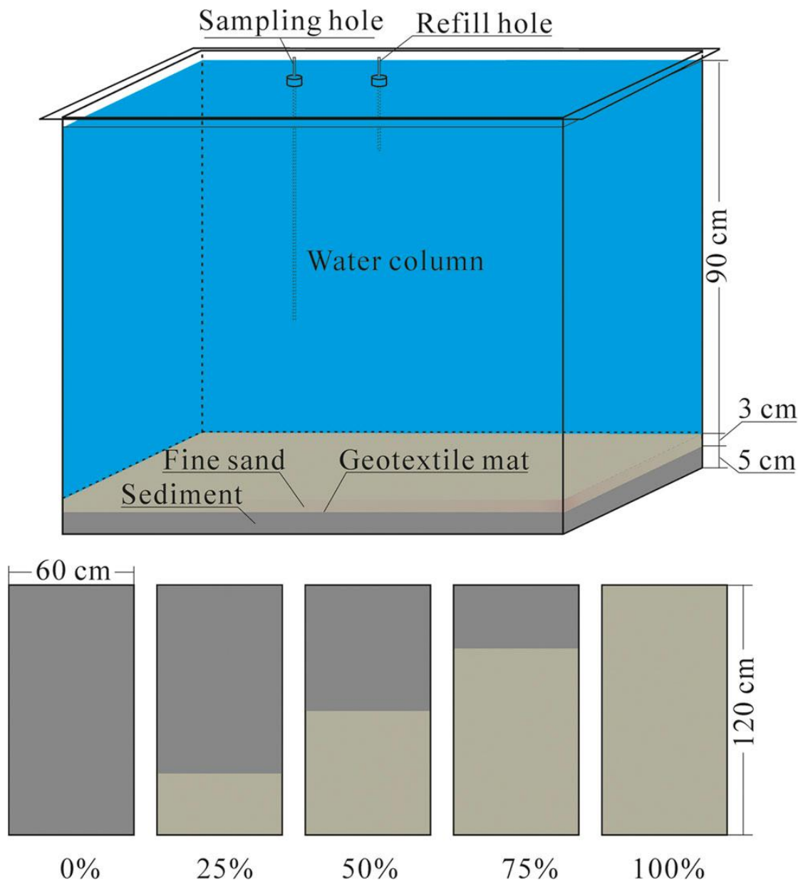
Fig. 1 Diagrams of the of the tanks used in the experiment (top) from the side and (bottom) from the top, showing the percentage coverage of fine sand used in the control (0%) and four treatments.
