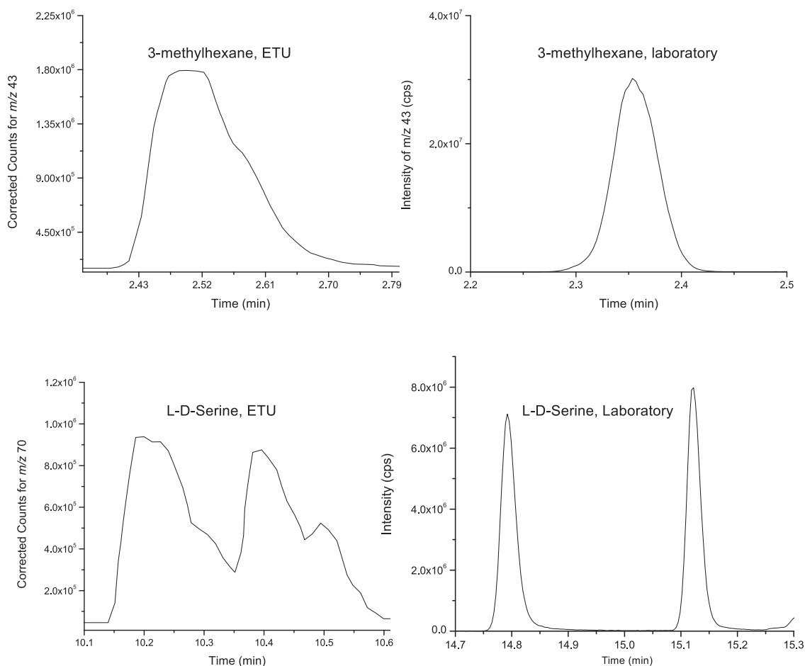
Fig. 10. Comparison of MOMA ETU separation of pure chiral 3-methylhexane (top left) and laboratory test (top right). Comparison of MOMA ETU separation of L-D-serine (bottom left) and laboratory test (bottom right). The m/z 43 ion is shown for methylhexane and the m/z 70 ion is shown for serine. For the ETU test, the GC column was held isothermally at 35 °C. For the laboratory test, the GC column was held at 35 °C for 7 min and then ramped to 182 °C at a ramp rate of 10 °C·min -1 .
