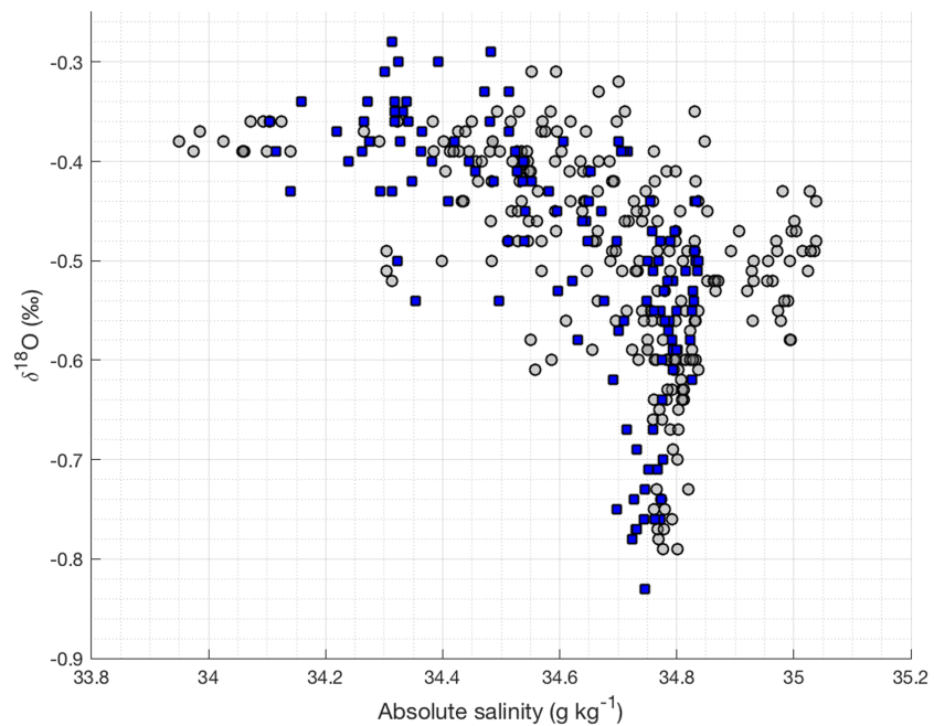
Figure A1. \delta^{18}\text{O}-S_A characteristics of (blue squares) observations sampled in front of Filchner Ice Shelf in 2017 (observations corresponding transects shown in Figure 2a) and (gray circles) observations sampled in front of FRIS in 1995 (observations corresponding to the transects shown in Figure 2f).
