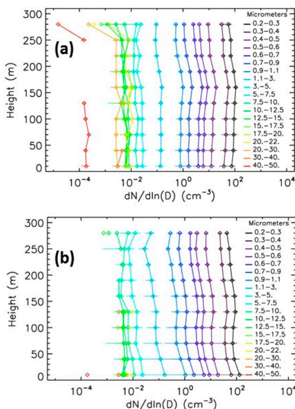
Figure 7. Evolution with height of number concentrations for the 19 size classes of LOAC when the urban pollution is low. (a) 8 July 2016; (b) 20 September 2017.
