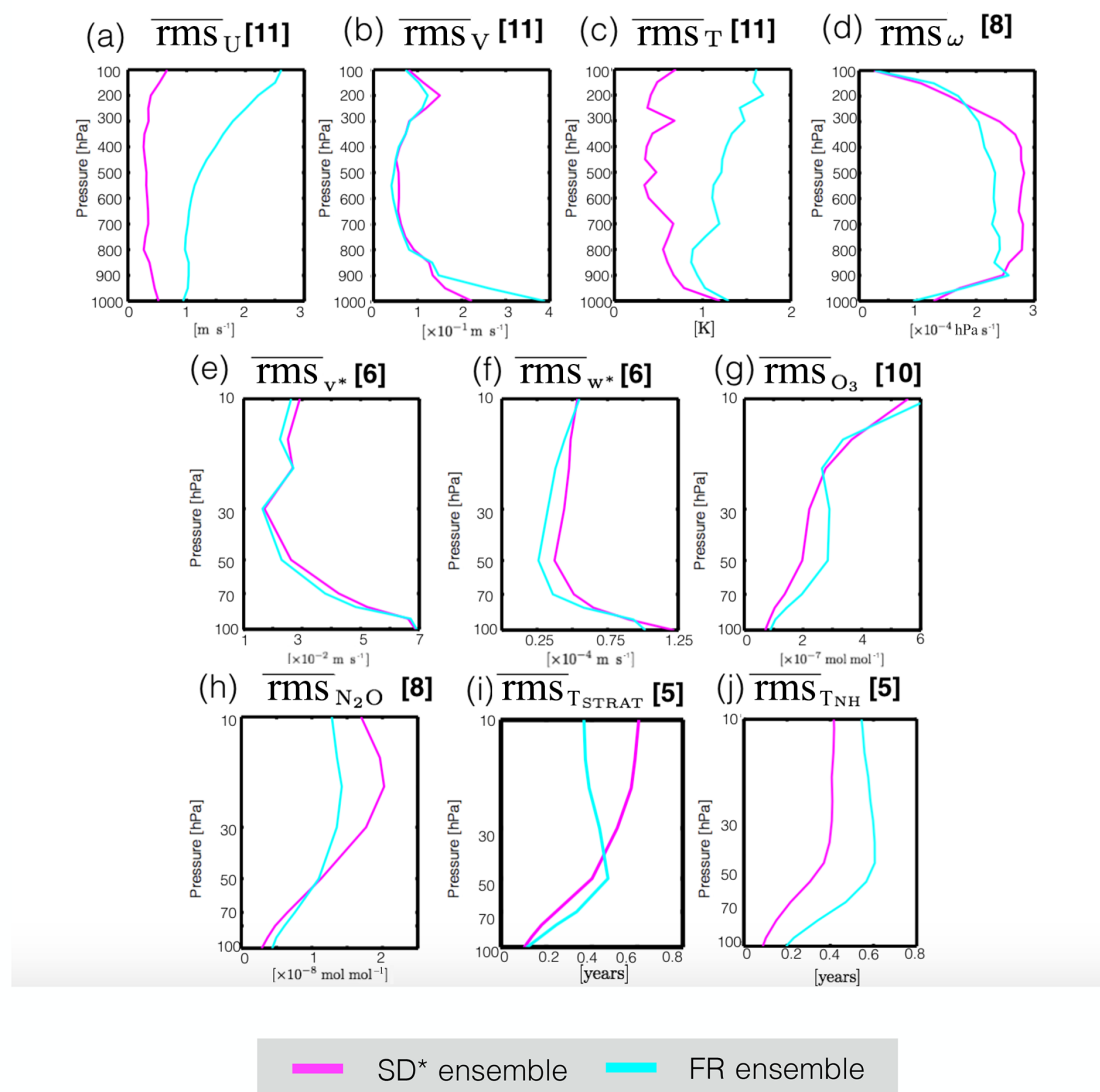
Figure 10. The root-mean-square (rms) spread of the (a) zonal mean zonal winds, (b) zonal mean meridional winds, (c) zonal mean temperatures, (d) zonal mean pressure velocities, (e) residual mean horizontal velocity, (f) residual mean vertical velocity, (g) ozone, (h) nitrous oxide, (i) stratospheric mean age and (j) NH midlatitude mean age. The pink and cyan lines correspond to the ensemble mean rms spread evaluated over the SD* and FR ensembles, where the asterisk denotes the subset of SD simulations for which there was a corresponding free-running simulation (last column in Table 1).
