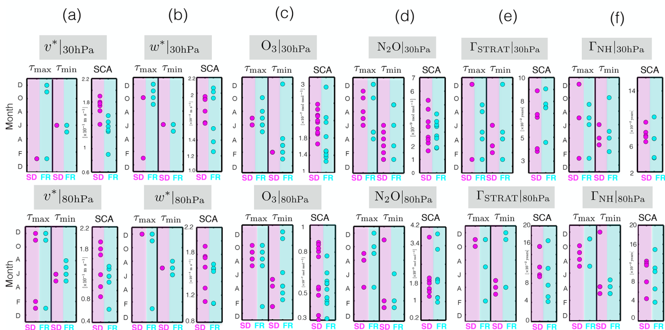
Figure 12. Same as Fig. 11 but now evaluated for the stratospheric dynamical and transport variables, shown here at 30 hPa (top) and 80 hPa (bottom).
