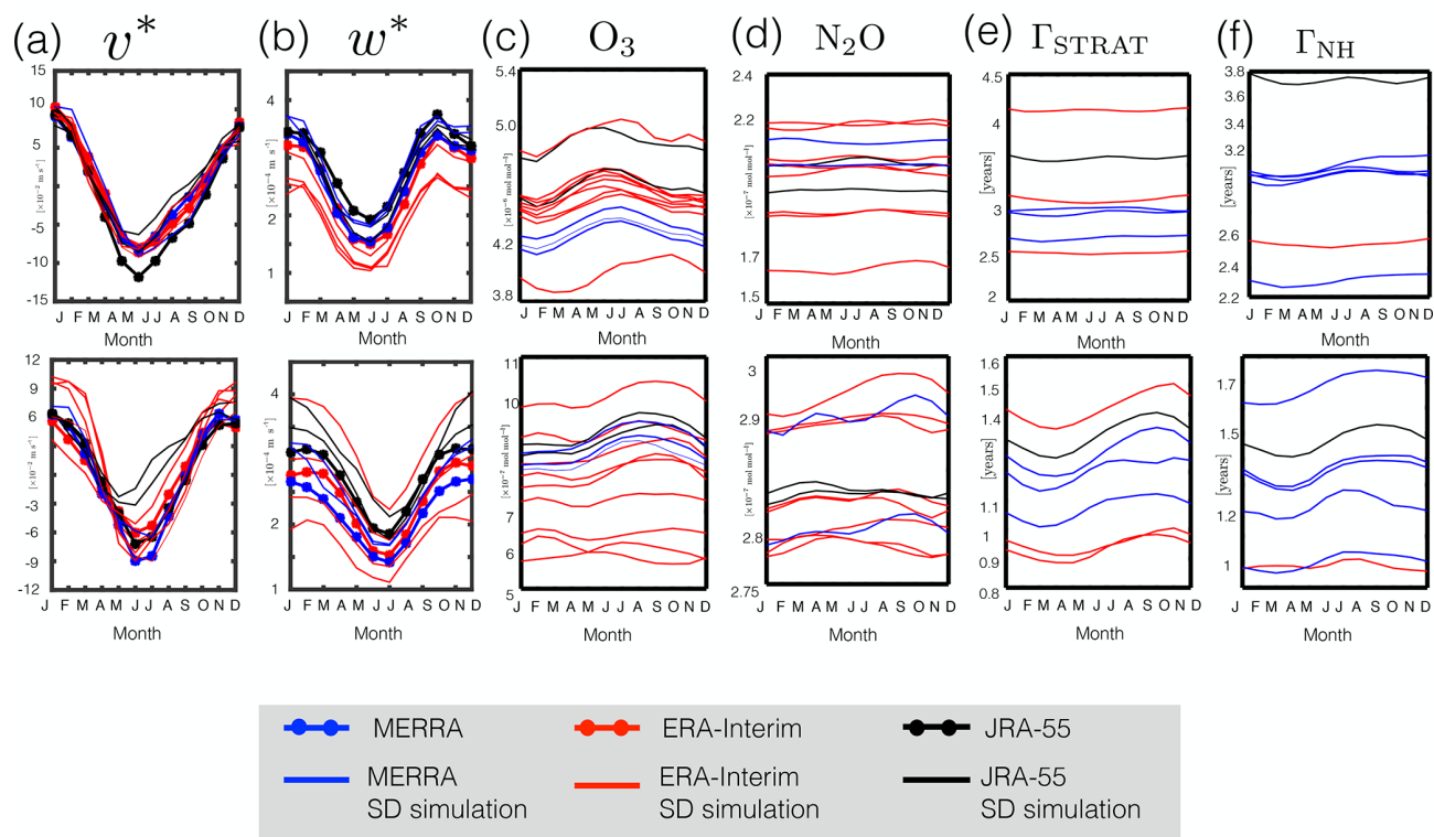
Figure 5. Same as Fig. 3 but now for the stratospheric dynamical and transport diagnostics. Shown are the 2000–2009 climatological mean seasonal cycles of the (a) residual mean meridional velocity ( v^* ), (b) residual mean vertical velocity ( w^* ), (c) ozone ( O_3 ), (d) nitrous oxide ( N_2O ), (e) stratospheric mean age ( \Gamma_{STRAT} ) and (f) NH midlatitude mean age ( \Gamma_{NH} ). The seasonal cycle is shown at 30 hPa (top panels) and 80 hPa (bottom panels), and all latitudinal averages have been performed over 60^\circ S and 60^\circ N ( 30^\circ S and 30^\circ N for w^* ). For the cases of v^* and w^* red/blue/black dotted lines correspond to the S-RIP TEM velocities derived from ERA-Interim/MERRA/JRA-55 meteorological fields.
