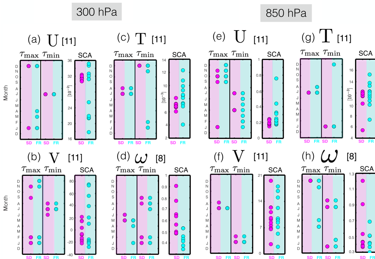
Figure 11. Same as Fig. 4 but now evaluated for the SD* and FR ensembles in pink and cyan, respectively. Note that both ensembles contain the same number of ensemble members per variable, as shown in the title within each panel.
