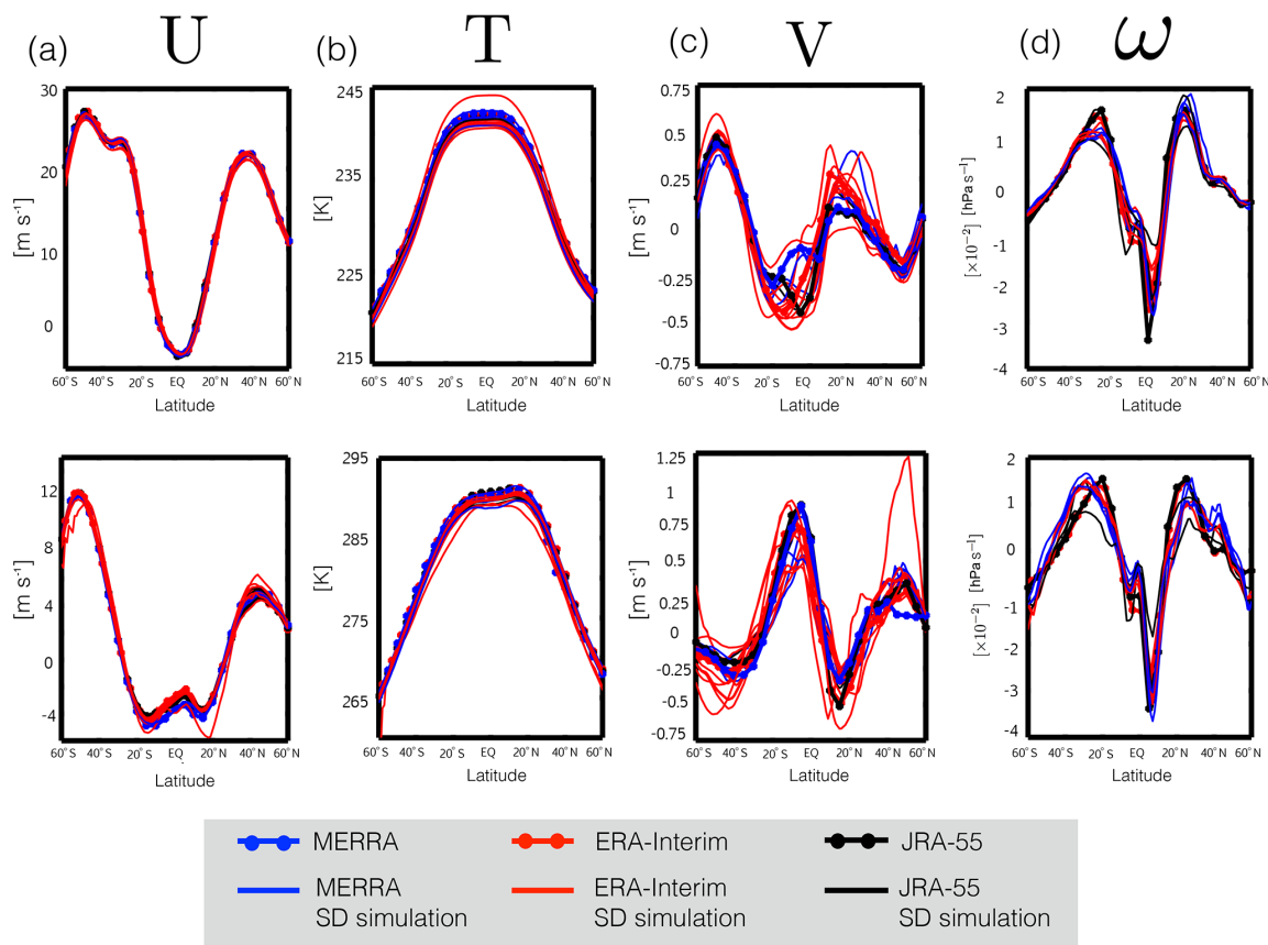
Figure 1. Meridional profiles of the 2000–2009 climatological annual mean (a) zonal mean zonal wind ( U ), (b) zonal mean temperature ( T ), (c) zonal mean meridional wind, and (d) zonal mean pressure velocity ( \omega ) at 300 hPa (top panels) and 850 hPa (bottom panels). Red/blue/black lines correspond to SD simulations constrained with ERA-Interim/MERRA/JRA-55 reanalysis fields. Red/blue/black dotted lines correspond to the raw ERA-Interim/MERRA/JRA-55 meteorological fields. Note that MERRA assimilated fields are shown, for which \omega is not available.
