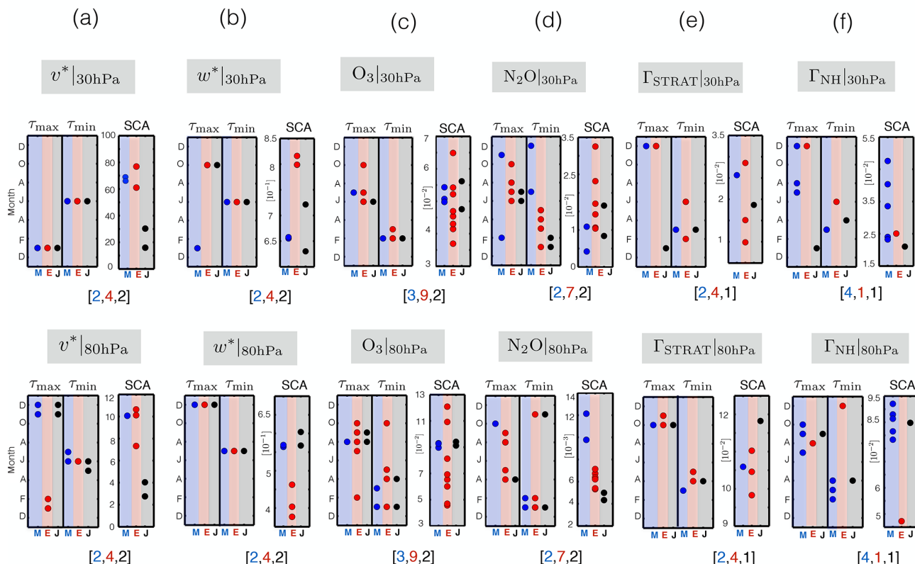
Figure 6. Same as Fig. 4 but now for the stratospheric dynamical and transport diagnostics.
