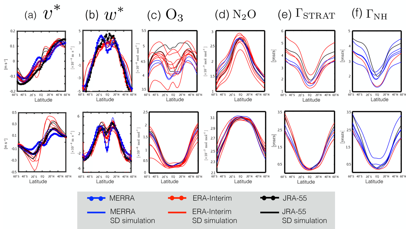
Figure 2. Meridional profiles of the 2000–2009 climatological annual mean (a) residual meridional velocity ( v^* ), (b) residual vertical velocity ( w^* ), (c) ozone ( O_3 ), (d) nitrous oxide ( N_2O ), (e) stratospheric mean age ( \Gamma_{STRAT} ) and (f) Northern Hemisphere midlatitude mean age ( \Gamma_{NH} ). Profiles are shown for 30 hPa (top) and 80 hPa (bottom). Red/blue/black lines correspond to SD simulations constrained with ERA-Interim/MERRA/JRA-55 reanalysis fields. For the cases of v^* and w^* red/blue/black dotted lines correspond to the S-RIP TEM velocities derived from ERA-Interim/MERRA/JRA-55 meteorological fields.
