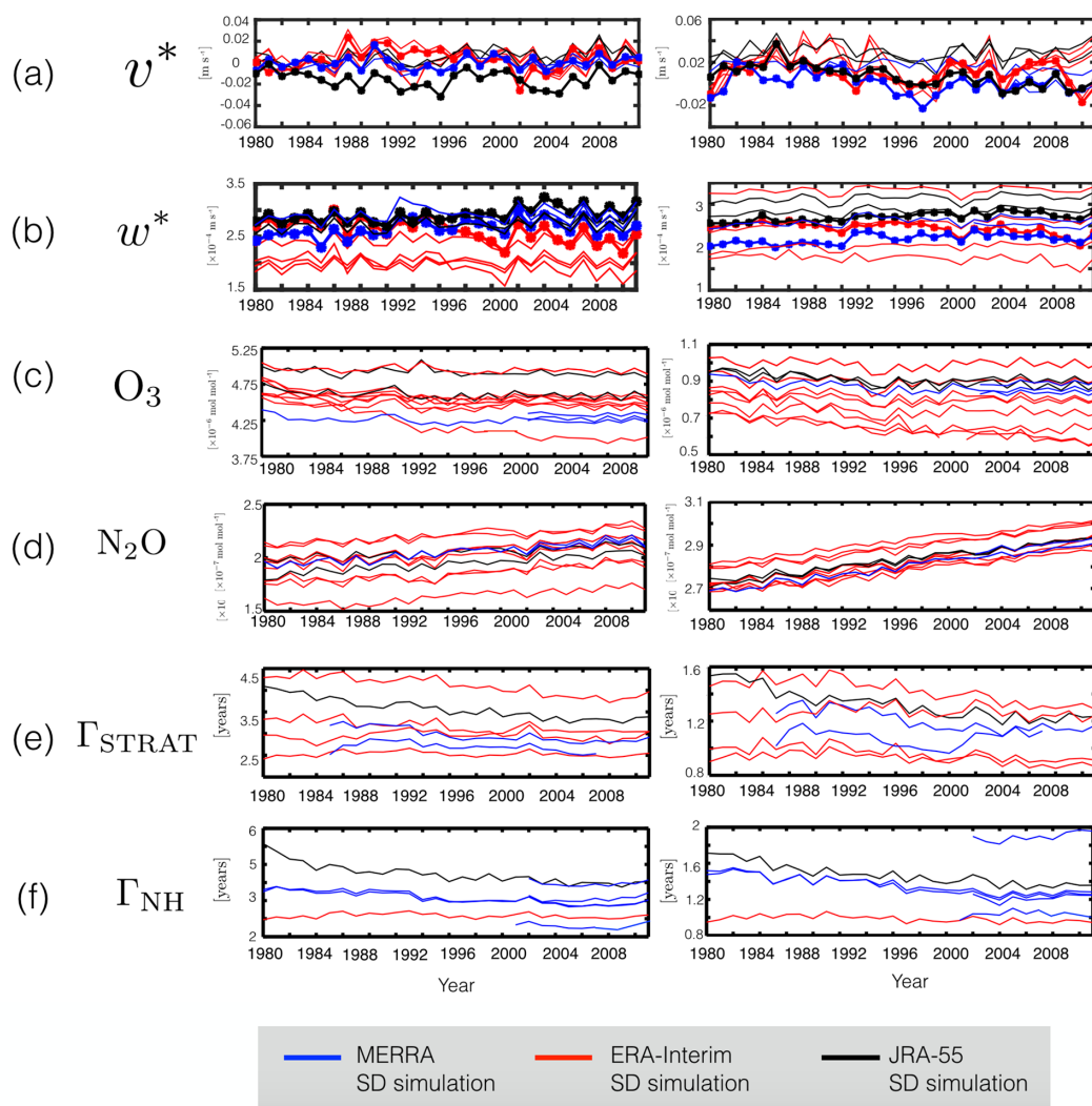
Figure 8. Same as Fig. 7 but for the stratospheric dynamical and transport fields, evaluated at 30 hPa (left) and 80 hPa (right). For the cases of v^* and w^* red/blue/black dotted lines correspond to the S-RIP TEM velocities derived from ERA-Interim/MERRA/JRA-55 meteorological fields.
