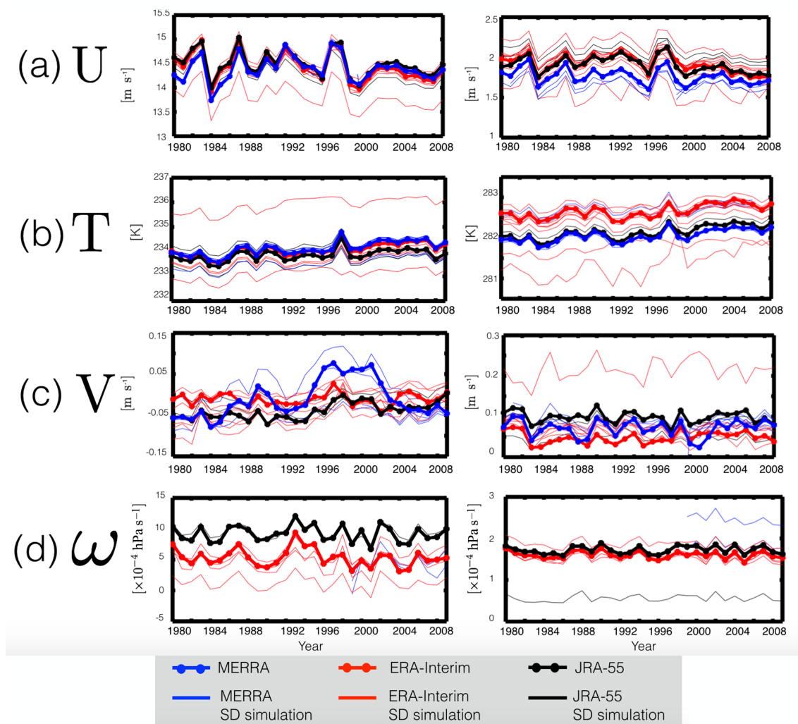
Figure 7. Time series of the zonal mean zonal winds (a), zonal mean temperatures (b), zonal mean meridional winds (c), and zonal mean vertical velocities (d) at 300 hPa (left panels) and 850 hPa (right panels). Red/blue/black solid lines correspond to SD simulations constrained with ERA-Interim/MERRA/JRA-55 reanalysis fields. Red/blue/black dotted lines correspond to the raw ERA-Interim/MERRA/JRA-55 meteorological fields. MERRA assimilated fields are shown for all variables, except for \omega , for which output was not available.
