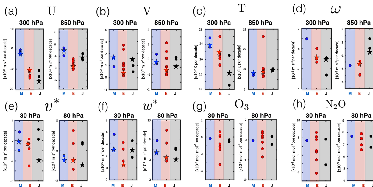
Figure 9. Top: trends in the zonal mean zonal winds (a), meridional winds (b), temperatures (c) and pressure velocities (d), evaluated as simple linear fits of the time series shown in Fig. 7 over years 1980–2009. Bottom: same but for the (e) residual mean meridional velocity, (f) residual mean vertical velocity, (g) ozone and (h) nitrous oxide. Red/blue/black circles denote the SD simulations, whereas the stars refer to the trends inferred directly from the S-RIP TEM velocities derived from ERA-I/MERRA/JRA-55 reanalysis fields.
