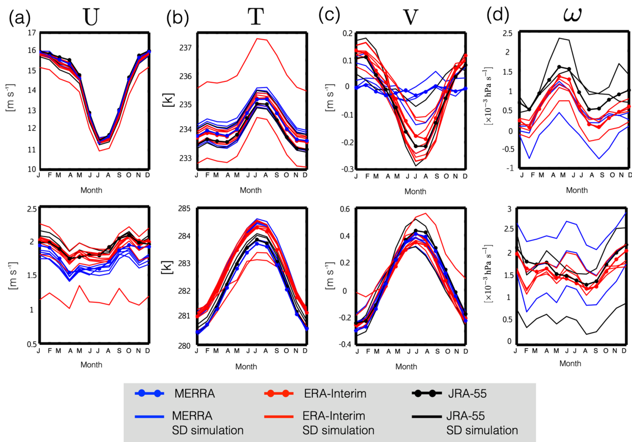
Figure 3. The 2000–2009 climatological mean seasonal cycle of the (a) zonal mean zonal wind ( U ), (b) zonal mean temperature ( T ), (c) zonal mean meridional wind ( V ), and (d) zonal mean pressure velocity ( \omega ) at 300 hPa (top panels) and 850 hPa (bottom panels). Seasonal cycles have been averaged over latitudes spanning 60^\circ S and 60^\circ N ( 30^\circ S and 30^\circ N for \omega ). Red/blue/black solid lines correspond to SD simulations constrained with ERA-Interim/MERRA/JRA-55 reanalysis fields. Red/blue/black dotted lines correspond to the raw ERA-Interim/MERRA/JRA-55 meteorological fields. As in Fig. 1 note that MERRA assimilated fields are shown, for which \omega is not available.
