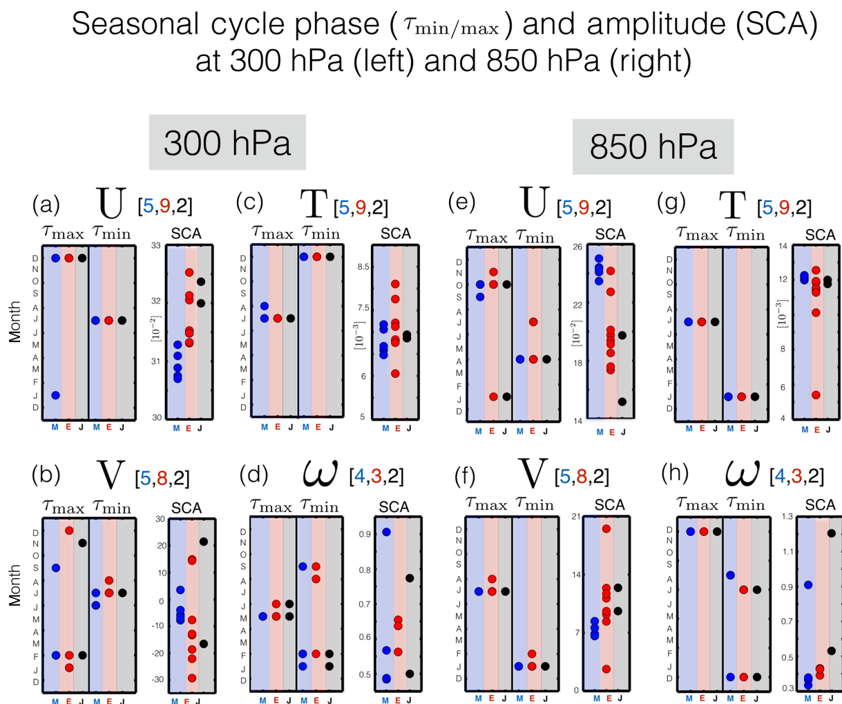
Figure 4. The seasonal cycle phase, represented in terms of \tau_{\min} and \tau_{\max} , and seasonal cycle amplitude (SCA) of the zonal mean zonal winds (a, e), zonal mean temperatures (c, g), zonal mean meridional winds (b, f) and zonal mean pressure velocities (d, h). Each dot represents an individual model simulation. The seasonal cycle amplitude has been normalized by the climatological mean annually averaged value for each variable shown. Red/blue/black circles show the spread among the SD simulations constrained with ERA-I/MERRA/JRA-55 reanalysis fields. Panels (a–d) and (e–h) correspond to evaluations at 300 and 850 hPa, respectively. Note that the number of ensemble members per ensemble and for each variable are shown in the title within each panel. In addition, note that in several panels only a few dots are visible. This reflects the overall good consistency in the seasonal cycle phase among the simulations.
