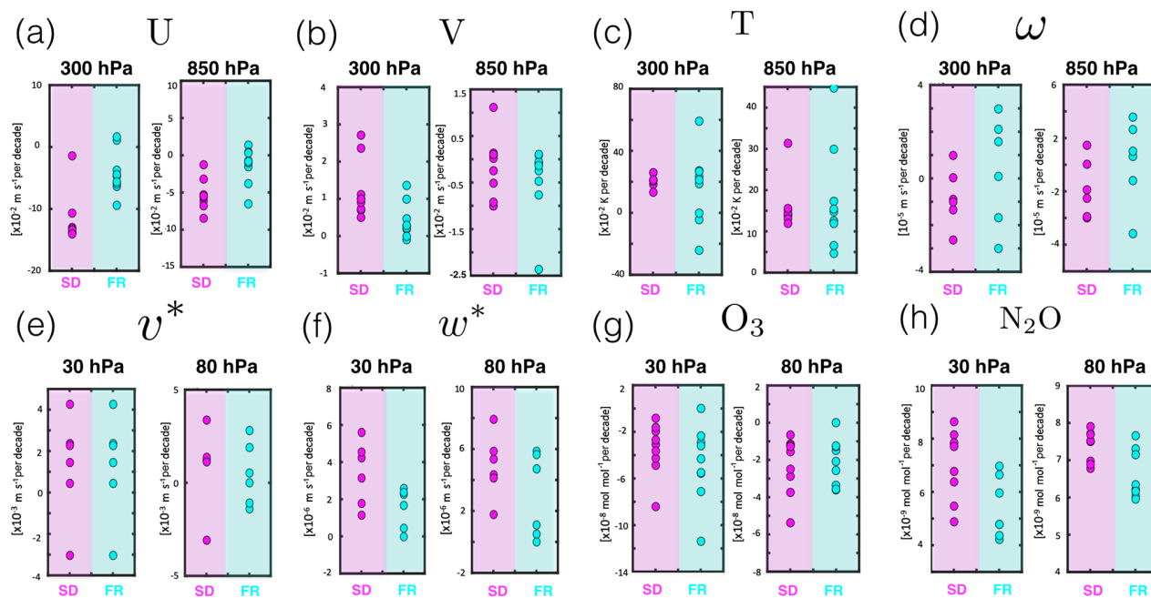
Figure 13. Same as Fig. 9 but now evaluated for the SD* and FR ensembles in pink and cyan.
