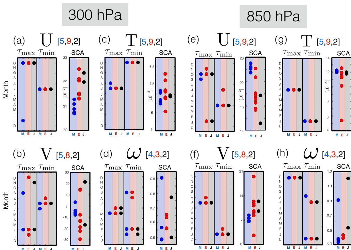
Figure 4. The seasonal cycle phase, represented in terms of \tau_{\min} and \tau_{\max} , and seasonal cycle amplitude (SCA) of the zonal mean zonal winds (a, e), zonal mean temperatures (c, g), zonal mean meridional winds (b, f) and zonal mean pressure velocities (d, h). Each dot represents an individual model simulation. The seasonal cycle amplitude has been normalized by the climatological mean annually averaged value for each variable shown. Red/blue/black circles show the spread among the SD simulations constrained with ERA-I/MERRA/JRA-55 reanalysis fields. Panels (a–d) and (e–h) correspond to evaluations at 300 and 850 hPa, respectively. Note that the number of ensemble members per ensemble and for each variable are shown in the title within each panel. In addition, note that in several panels only a few dots are visible. This reflects the overall good consistency in the seasonal cycle phase among the simulations.
