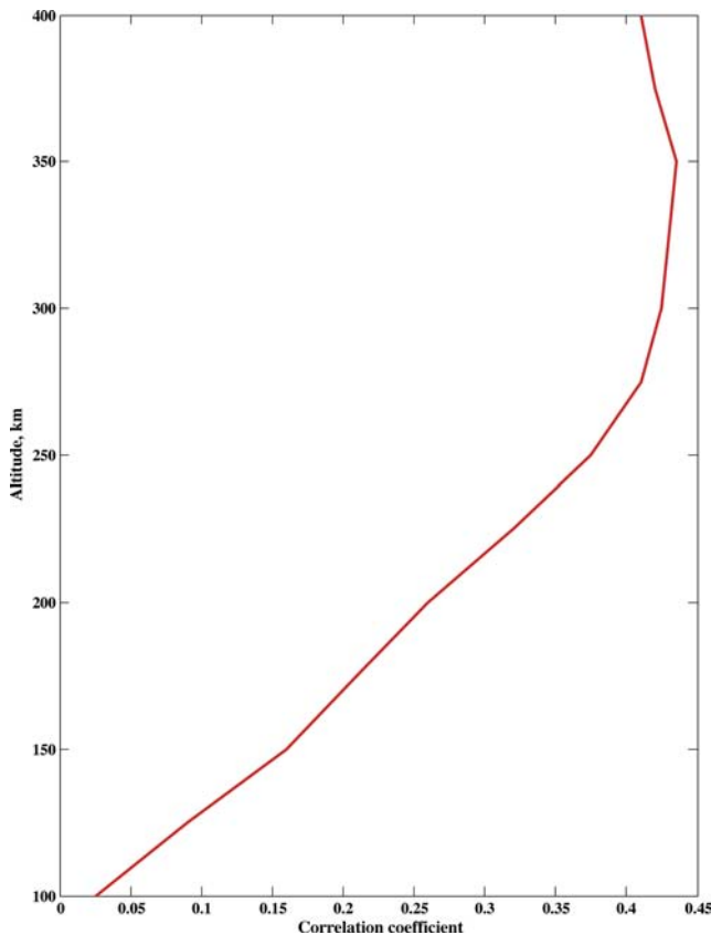
Figure 5. The altitude variation of average correlation coefficient deduced from the GPS observation during Denali earthquake.
