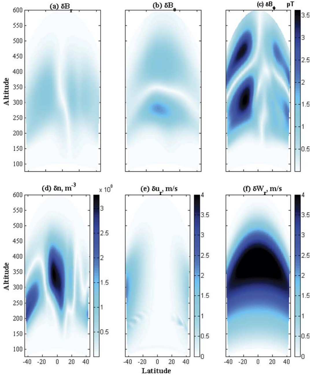
Figure 4. (a–c) The distribution of three components of fluctuating magnetic field \delta\vec{B} , (d) density fluctuations \delta n , (e) perturbed radial velocity of electron \delta u_r^e and (f) perturbed radial wind \delta W_r .
