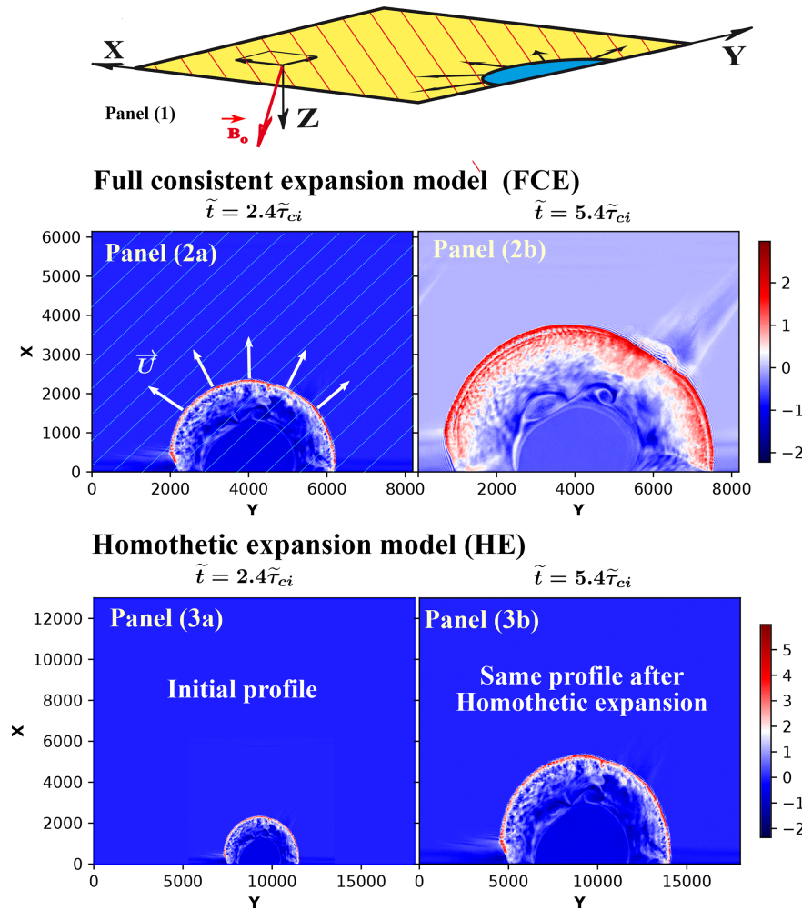
Figure 1. Panel (1) plots the simulation plane geometry; the \tilde{B}_o magnetostatic field is mainly outside and directed downward from the plane. Panels (2a, b) illustrate the evolution of the magnetic field \tilde{B}_{tz} in the fully consistent expansion (FCE) model (time dependent), respectively, at \tilde{t}_{init} = 2.4\tilde{\tau}_{ci} and \tilde{t}_{simul} = 5.4\tilde{\tau}_{ci} . In panel (2a), used as a reference, the vector velocity \tilde{U} = \tilde{v}_{shock} has been superimposed to illustrate the shock front propagation (white thick arrows); the arrow length is not at the right scale. In addition, the projection of the \tilde{B}_o magnetic field lines has been reported (oblique white thin lines). Panels (3a, b) illustrate one example of the curved magnetic field \tilde{B}_{tz} in the homothetic expansion (HE) model (time independent), where the shock profile is fixed in time but expands in space via an expanding factor proportional to the shock front velocity v_{shock} \times t ; this shock profile has been chosen at the time \tilde{t}_{init} = 2.4\tilde{\tau}_{ci} of the self-consistent simulation. From this time, the shock front dilates by a factor of 2.6 compared to its initial shape.
