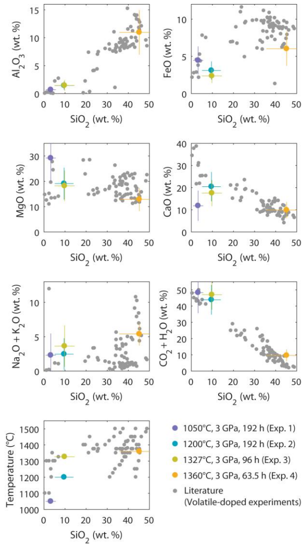
Fig. 4. Composition of incipient melts in a (CO 2 +H 2 O)-bearing mantle rock experimentally re-equilibrated at shallow mantle temperatures and pressure. Literature data regroup experiments producing volatile-bearing melts (CO 2 and/or H 2 O) at comparable pressures (2.5-3.5 GPa) and temperatures (up to 1500°C), in at least CaO-MgO-Al 2 O 3 -SiO 2 -FeO systems and where melts equilibrate with at least olivine and orthopyroxene. See Table S1 for literature data selection.
