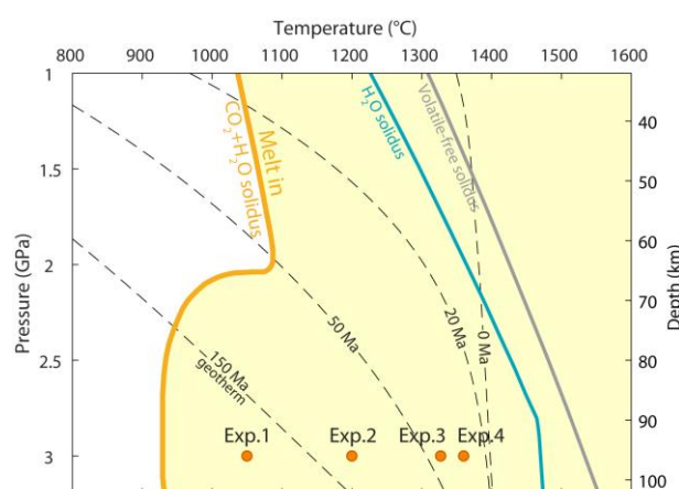
Fig. 1. Incipient melting at shallow mantle temperatures and pressure. Present experiments investigate the domain of (\text{CO}_2+\text{H}_2\text{O}) -assisted melting (Wallace and Green, 1988) which covers young and hot to old and cold oceanic mantle, down to temperatures where both volatile-free-melting and \text{H}_2\text{O} -only-melting (200 wt.ppm) (Sarafian et al., 2017) are precluded. Mantle thermal structure is G13R1350 model with 1350^\circ\text{C} potential temperature from Grose and Afonso (2013).
