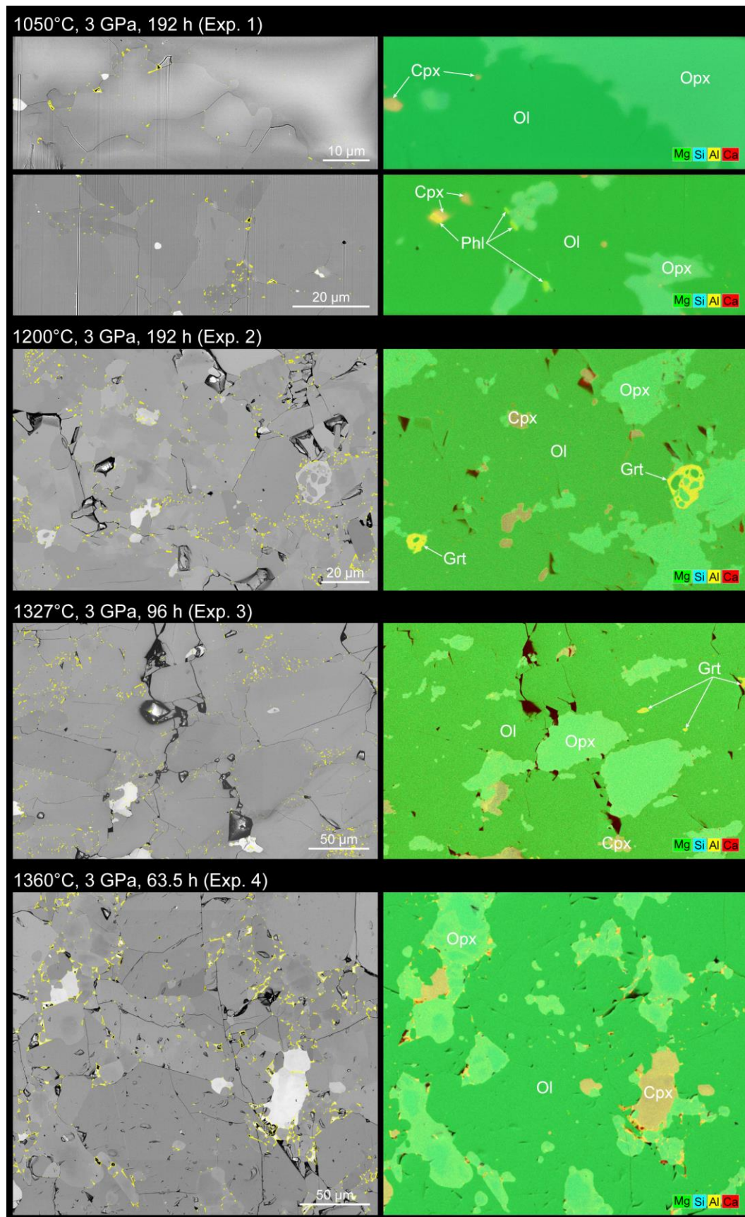
Fig. 2. Broad image and chemical mappings of a (CO 2 +H 2 O)-bearing mantle rock experimentally re-equilibrated at shallow mantle temperatures and pressure. Left panels, backscattered electron image mappings on which melt contours are reported in
