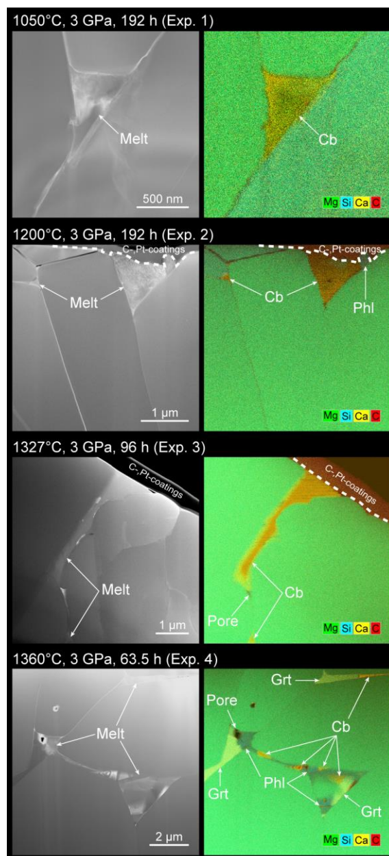
Fig. 3. High magnification imaging and chemical mappings of incipient melts in a (CO 2 +H 2 O)-bearing mantle rock experimentally re-equilibrated at shallow mantle temperatures and pressure. Left panels, transmission electron imaging of electron-transparent thin sections extracted perpendicular to sample surfaces. Right panels, corresponding chemical mappings reported as superposition of magnesium, silicon, calcium and carbon EDS maps. Note that the melt does not quench as glass at the end of the experiments but results in quenched nano-crystals and fluid-filled pores (Cb = carbonate, Phl = phlogopite, Grt = garnet).
