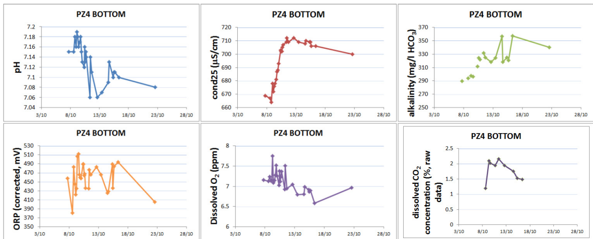
Fig. 4. Evolution of pH, electrical conductivity, alkalinity – expressed as bicarbonate content, redox potential (ORP), dissolved oxygen and raw dissolved \text{CO}_2 concentrations at 18 m depth in PZ4.
