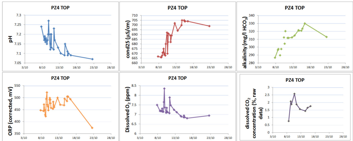
Fig. 3. Evolution of pH, electrical conductivity, alkalinity – expressed as bicarbonate content, redox potential (ORP), dissolved oxygen and raw dissolved \text{CO}_2 concentrations at 15 m depth in PZ4.
