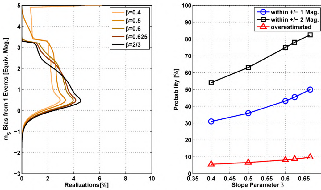
1226 Figure 10 NLVR estimator marginal distribution densities for different slope parameters. Left: the marginal distribution 1227 densities for all catalogs (corresponding to the grey curve in Figure 8). Each curve represents approx. 8 million evaluated 1228 catalogs. Right: percentage of estimations that are within \pm 1 (blue) or \pm 2 magnitudes (black) from the true moment rate, 1229 and the fraction of overestimated moment rates (red).
