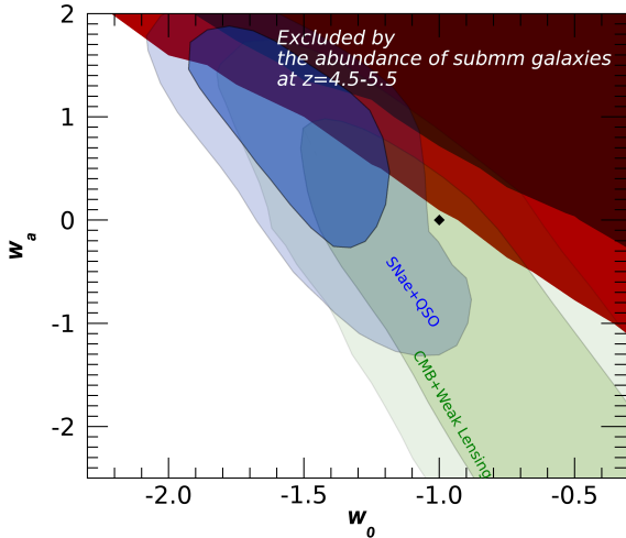
Fig. 4. Exclusion regions (2- \sigma confidence level) in the w_0 - w_a plane (see text) derived from the observed abundance \phi_{obs} of luminous submm galaxies at z = 4.5 - 5.5 (Wang et al. 2019). The brown region corresponds to assuming the observed stellar masses M_* = M/f_b to be related to the DM mass through the baryon fraction f_b . The red regions corresponds to adopting the DM mass derived from the measured cross-correlation function of H-dropouts (see text).
