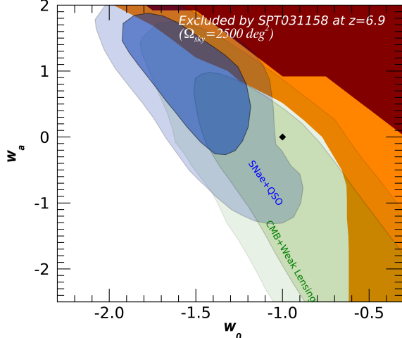
Fig. 5. Exclusion regions ( 2\text{-}\sigma confidence level) in the w_0 - w_a plane (see text) for two different inferred DM mass of SPT031158: 2 \cdot 10^{12} M_{\odot} (red area) and 6 \cdot 10^{12} M_{\odot} (yellow area). In both cases the full SPT survey area \Omega_{sky} = 2500 \text{ deg}^2 has been assumed.
