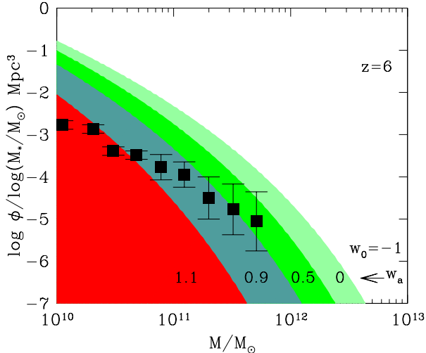
Fig. 1. The halo mass function at z = 6 predicted by different DDE models with w_0 = -1 and w_a = 0, 0.5, 0.9, 1.1 (from right to left, light green, green, dark green, and red colors, respectively). The black dots correspond to stellar mass function measured by Grazian et al. (2015) at z = 6 ; for the sake of simplicity, in this plot a conversion factor M_*/M = f_b has been assumed to assign a DM mass to the stellar mass of the measured data point.
