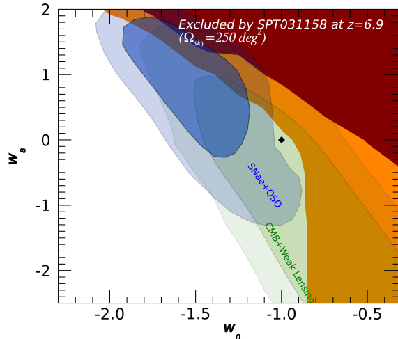
Fig. 6. Same as fig. 5, but assuming an effective SPT area \Omega_{sky} = 250 \text{ deg}^2 .
