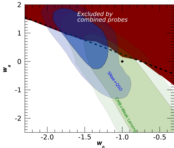
Fig. 7. Exclusion regions ( 2\text{-}\sigma confidence level) in the w_0 - w_a plane derived from combining the different probes. For each observable, the most conservative case has been considered: for the CANDELS field we have assumed F = 0.5 , for SPT031158 we have taken a DM mass M = 2 \cdot 10^{12} M_\odot , and for submm galaxies we have converted stellar masses to DM mass assuming M = M_*/f_b . The dashed line shows the analytical approximation for the boundary of the excluded region w_a = -3/4 - (w_0 + 3/2) .
