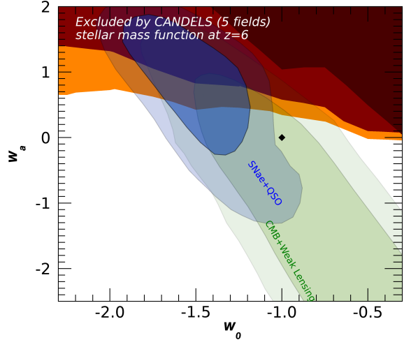
Fig. 3. As fig. 2, but assuming the errorbars of the stellar mass function reduced by 1/2 , to simulate the inclusion of the full set of CANDELS field. This improvement would exclude most of the region allowed by distant quasars.
