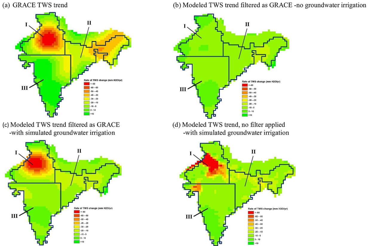
Fig. 5. Linear trends in observed and simulated TWS series.
