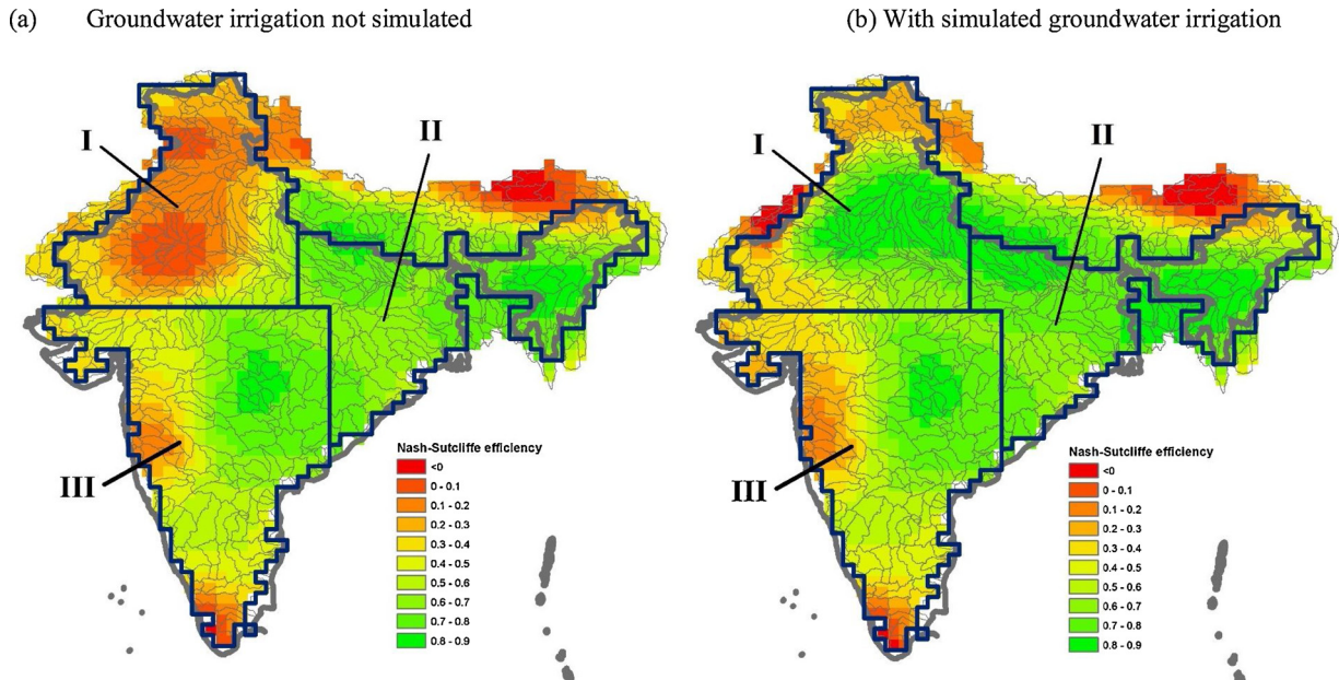
Fig. 4. A comparison of model fit between cases of (a) no simulation of groundwater irrigation and (b) groundwater irrigation simulation included (region I: northwest; region II: northeast & east; region III: central and south; the default values of five parameters included in the GLUE analysis to produce results shown in this figure, Figs. 5 and 6 are: water percolation rate in rice paddy = 8 mm H 2 O/day, threshold of upland crop water stress triggering irrigation = 0.7, Irrigation efficiency = 0.7, soil evaporation compensation factor = 0.95, groundwater recession coefficient = 0.05).
