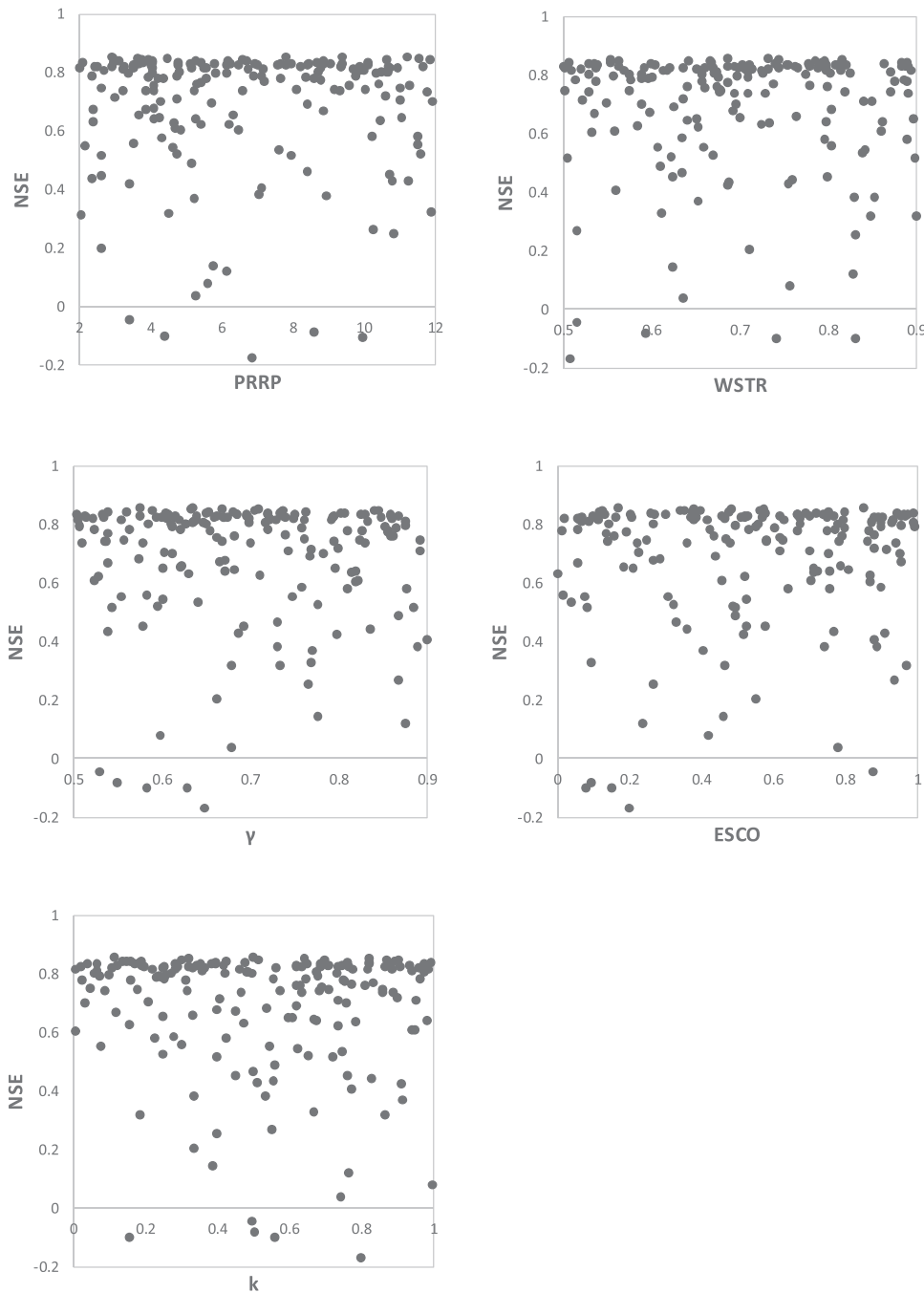
Fig. 8. Correspondence between sampled parameter values and the resultant NSE values indicating model fit over the northwest region of India obtained in Monte Carlo sampling. (Note: PRRP = water percolation rate for paddy rice; WSTR = threshold of upland crop water stress triggering irrigation; \gamma = irrigation efficiency; ESCO = soil evaporation compensation factor; k = groundwater recession coefficient).
