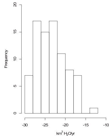
Fig. 9. Estimated annual averages of components of the groundwater balance in northwest India (July 2002–June 2011).
