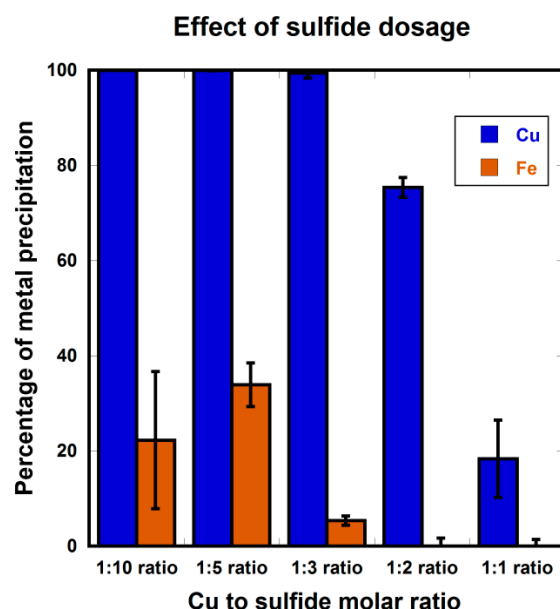
Figure 7. Effect of sulfide dosage on copper sulfide precipitation.
