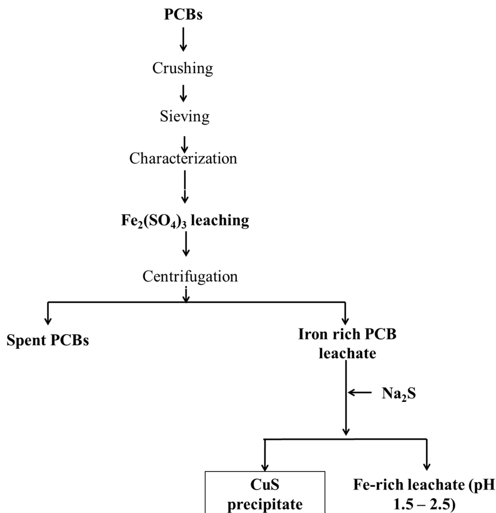
Figure 9. Hydrometallurgical flow chart for the selective recovery of Cu from PCBs.
