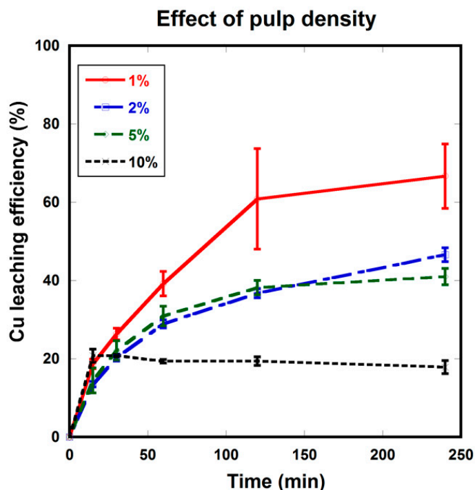
Figure 4. Effect of pulp density (Ferric sulfate—50 mM, Temperature—20 °C, and agitation—150 rpm).
