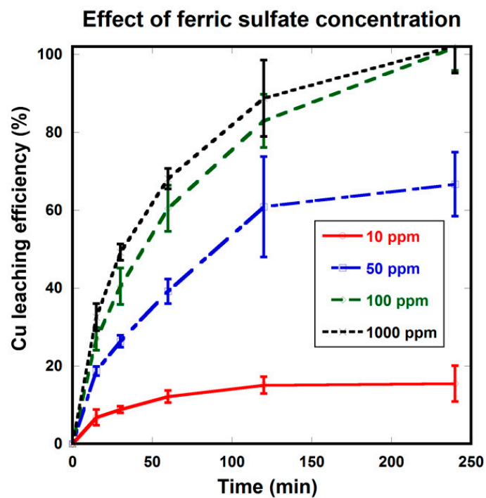
Figure 3. Effect of ferric sulfate concentration (Temperature—20 °C, agitation—150 rpm, and pulp density—10 g·L -1 ).
