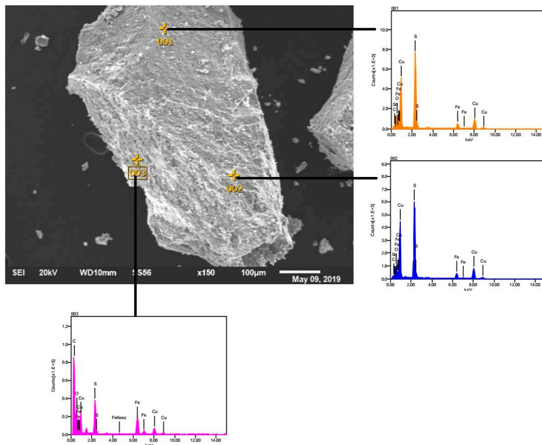
Figure 8. Scanning electron microscope–Energy dispersive X-ray spectroscopy (SEM-EDS) spectra of copper sulfide precipitate.
