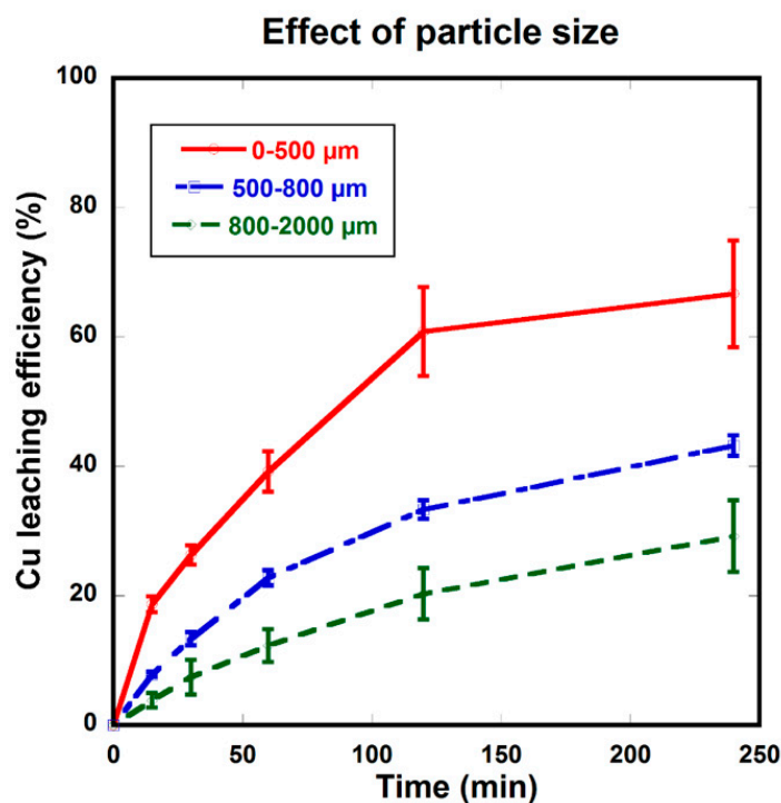
Figure 1. Effect of particle size (Ferric sulfate—50 mM, temperature—20 °C, agitation—150 rpm, and pulp density—10 \text{g}\cdot\text{L}^{-1} ).
