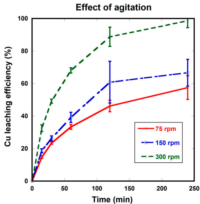
Figure 2. Effect of agitation (Ferric sulfate—50 mM, temperature—20 °C, and pulp density—10 g·L -1 ).
