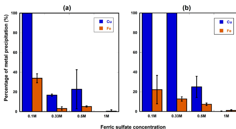
Figure 6. Effect of ferric sulfate concentration on copper sulfide precipitation. (a) Copper to sulfide ratio—1:5 and (b) Copper to sulfide ratio—1:10.
