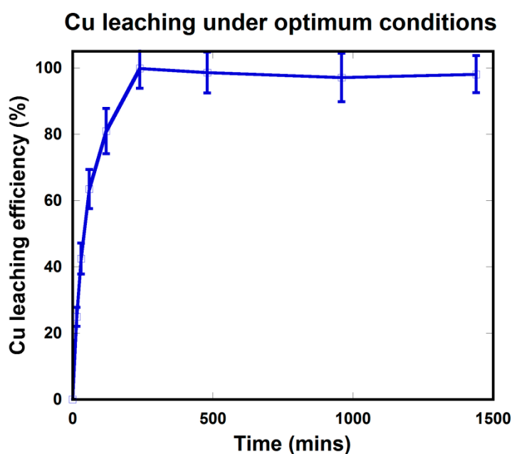
Figure 5. Leaching of Cu from PCBs under optimum conditions.
