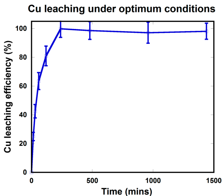
Figure 5. Leaching of Cu from PCBs under optimum conditions.
