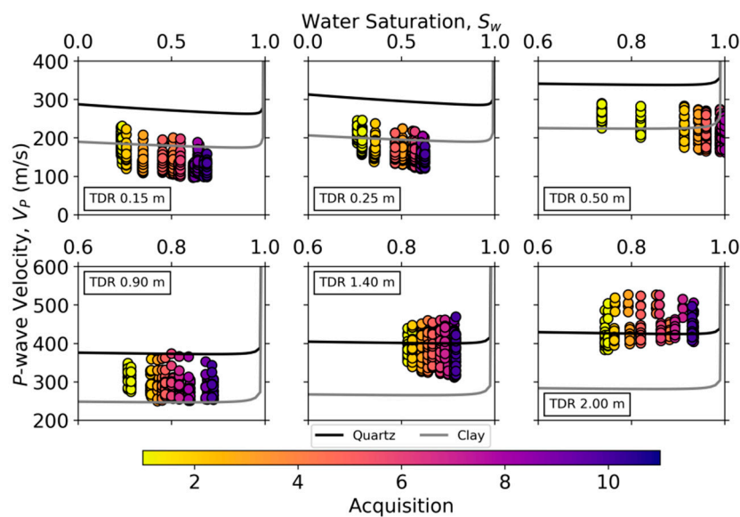
Figure 13. P-wave velocity ( V_p ) versus water saturation ( S_w ) inside the infiltration area at the depths of the TDR sensors. The solid lines correspond to velocity models described in the text for 100% quartz (black) and 100% clay (gray).
