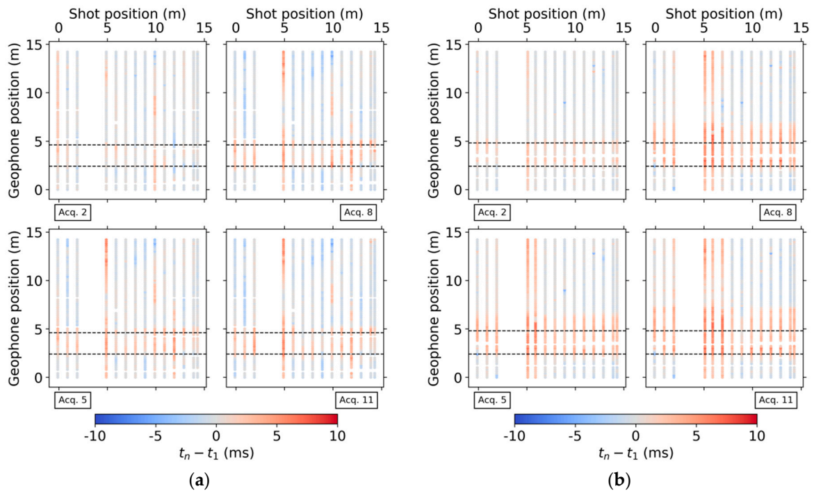
Figure 9. Picked traveltimes differences between the n th acquisition ( t_n , for n = 2, 5, 8, 11 ) and background acquisition ( t_1 ) for (a) NS and (b) WE lines for every shot-geophone pair. The black dashed lines delimit the geophone positions inside the infiltration area.
