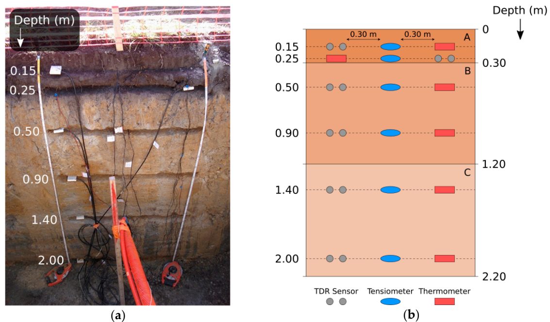
Figure 2. (a) Picture of the pit dug in 2012 with sensors installed [51]; (b) cross-section schematic showing sensor positions and horizons (A, B, C) described in Table 1.
