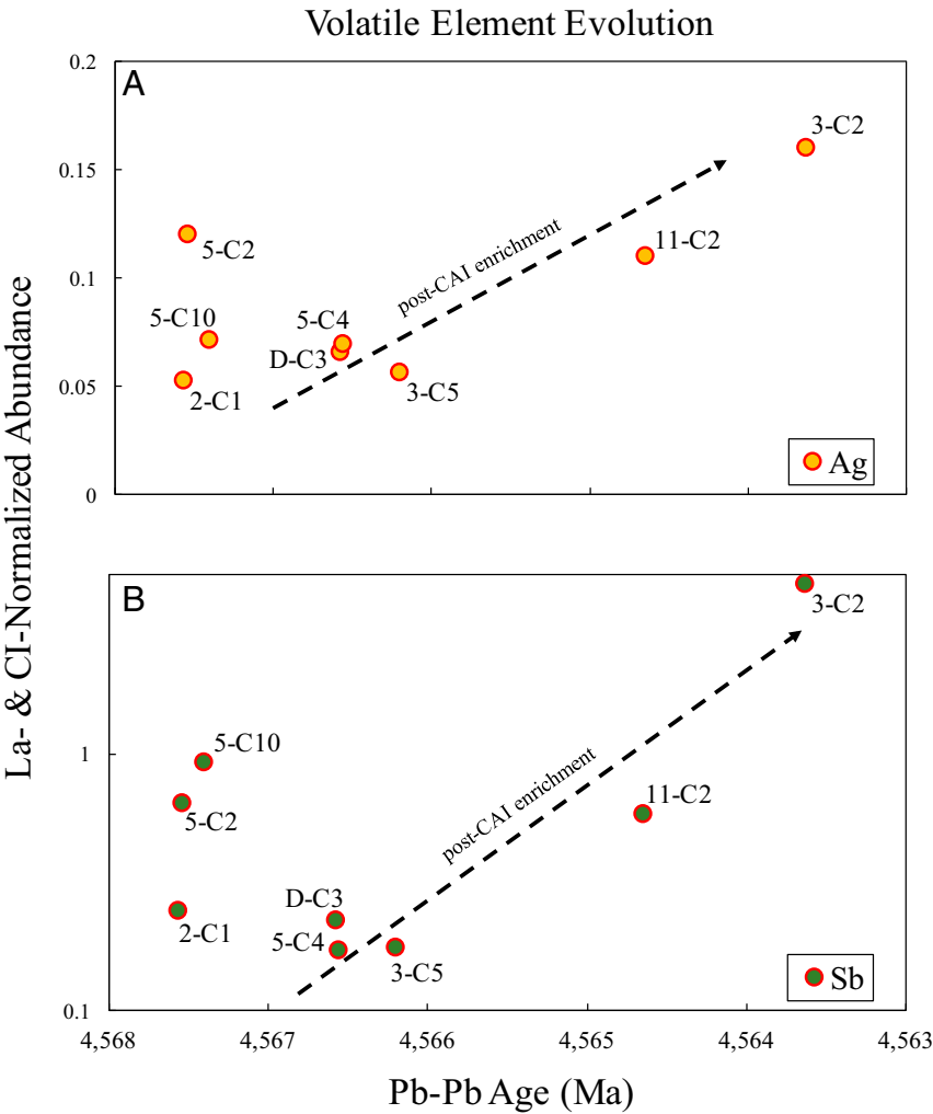
Fig. 2. La- and Cl-normalized (A) Ag and (B) Sb contents for L chondrite chondrules as a function of Pb–Pb age (17). General volatile enrichment through time indicates interaction of chondrules with a gas phase that is increasingly volatile-rich during recycling. Note the logarithmic scale for Sb in B.
