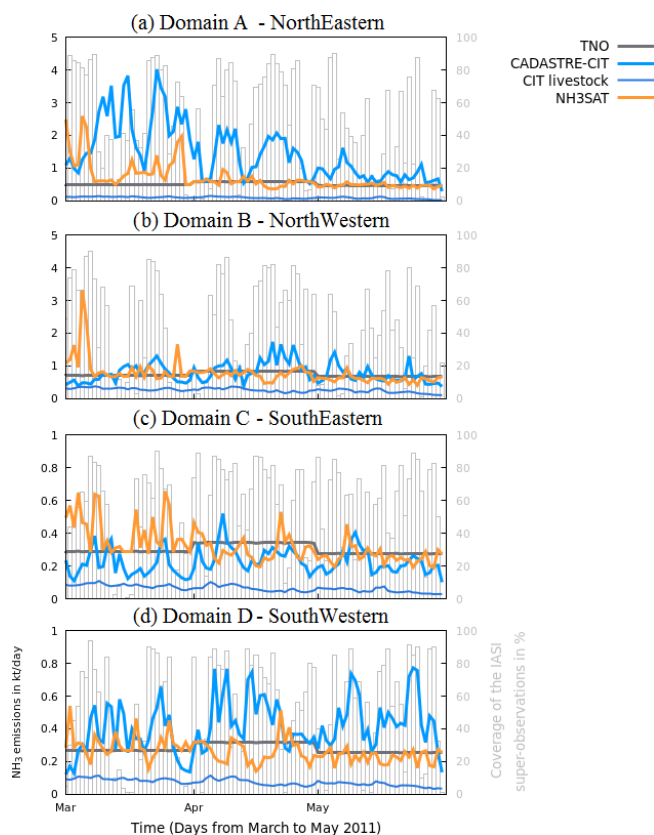
Figure 6. Time series of daily NH 3 emissions estimated by TNO-GEN (in black), by NH 3 SAT (in orange) and by CADASTRE-CIT (in blue) inventories, from March to May 2011, for (a) domain A (northeastern), (b) domain B (northwestern), (c) domain C (southeastern) and (d) domain D (southwestern), as defined in Fig. 2. Note that the scale is different between (a, b) and (c, d). Units are kilotons of NH 3 per day ( \text{kt NH}_3 \text{ d}^{-1} ). The contribution of the emissions due to livestock in the CADASTRE-CIT daily variability is also given. The daily regional coverage of the IASI super-observations is given in percentage (in grey).
