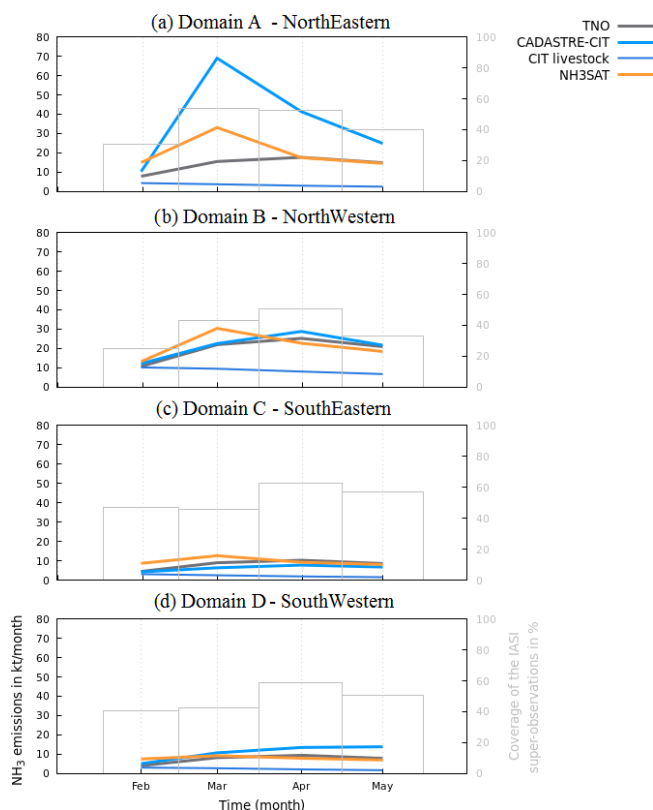
Figure 5. Time series of monthly NH 3 emissions estimated by TNO-GEN (in black), by NH 3 SAT (in orange) and by CADASTRE-CIT (in blue) inventories, from February to May 2011, for (a) domain A (northeastern), (b) domain B (northwestern), (c) domain C (southeastern) and (d) domain D (southwestern), as defined in Fig. 2. The contribution of the emissions due to livestock in the CADASTRE-CIT monthly budgets is also given. Units are kilotons of NH 3 per month ( \text{kt NH}_3 \text{ month}^{-1} ). The monthly regional coverage of the IASI super-observations is given in percentage (in grey).
