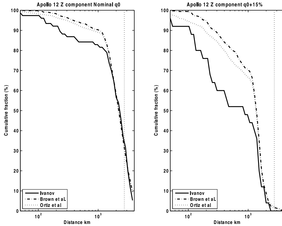
Figure 17. Cumulative percentage of impacts at a given epicentral distance for the (left) nominal and (right) high attenuation models. In the first case, about 30% of the events are found at epicentral distances greater than 90°, while this fraction is reduced to only a few percent in the high attenuation case. The high attenuation model reduces the amplitudes by a factor of up to 10 at epicentral distances of 2500 km (82°) and by 20 at 4000 km (132°).
