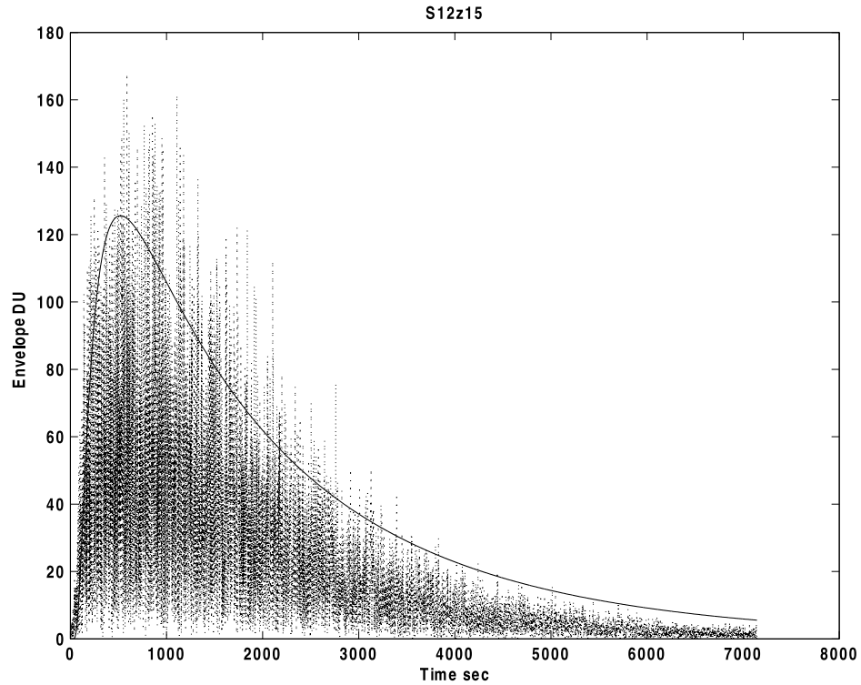
Figure 8. Typical waveform envelope fit, shown here for the impact of the Apollo 15 SIVB as recorded by the station 12 LP vertical component (epicentral distance of 355 km). In order to get more stable results, we fit the theoretical envelope using the median value between the running maximum of the envelope and its running mean value (in both cases defined for a window length of 300 s). The best fit was obtained by exploring the model space for all acceptable values of q , \alpha , \sigma , and A ; the residual misfit is typically a few percent.
