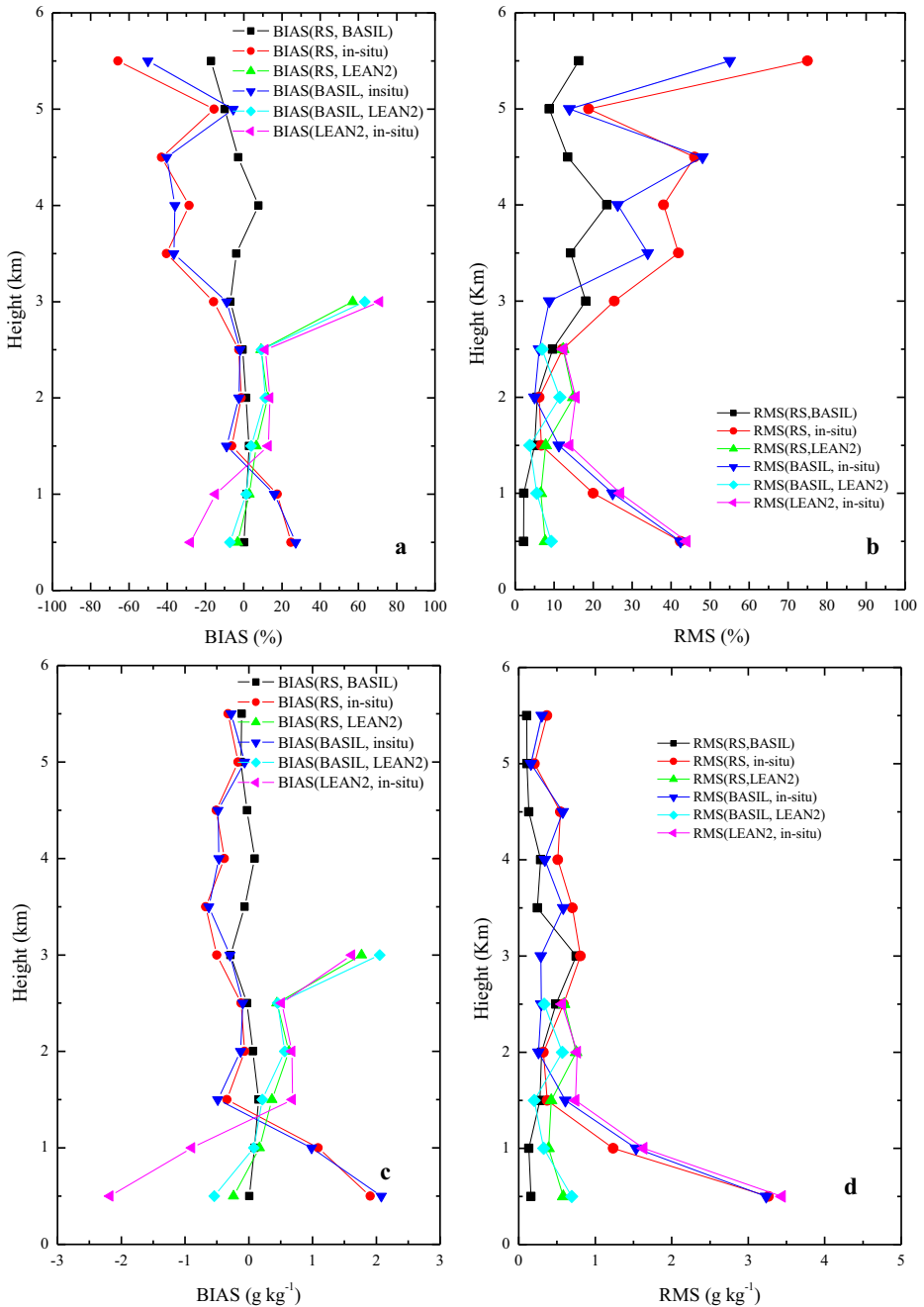
Fig. 9 BIAS (panels a and c ) and RMS deviation (panel b and d ) for the different sensors' pairs at 19:44 UTC on 02 October 2012. For the purpose of the comparisons in panels a–d , for BASIL, we considered the integration time 19:44–19:47 UTC, while for the in situ hygrometer, we considered the integration time 19:42–20:24 UTC
