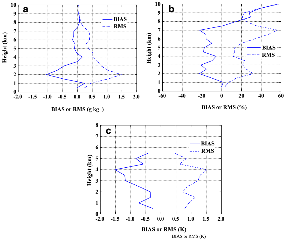
Fig. 15 Mean BIAS and RMS deviation profiles for the radiosondes vs. the MWR in terms of water vapor mixing ratio (panels a and b) and temperature (panel c)
