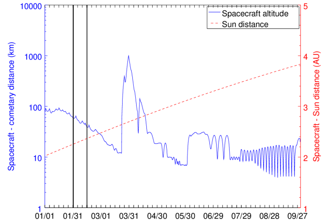
Fig. 5. Spacecraft-comet distance and Sun-spacecraft distance from January to September 2016. The vertical lines indicate when the spacecraft crossed the diamagnetic cavity (no magnetic field) that surrounded the comet nucleus (eight crossings on 31 January 2016, one crossing on 14 February 2016, and one crossing on 15 February 2016, each of them lasting less than 8 min).
