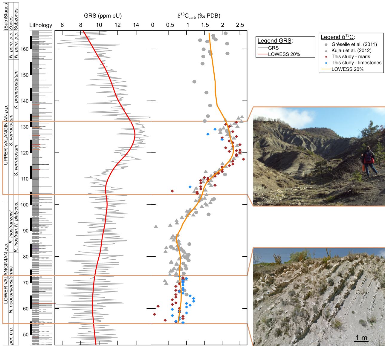
Figure 3. Vergol-Morénas composite section showing the log of the section, the gamma ray spectrometry (GRS) available in Martinez et al. (2013), the \delta^{13}C curves from Gréselle et al. (2011), Kujau et al. (2012), and this study (blue and brown diamonds), and the pictures of the two sequences of the Vergol-Morénas section studied here. LOWESS = LOcally WEighted Scatterplot Smoothing (Cleveland, 1979).
