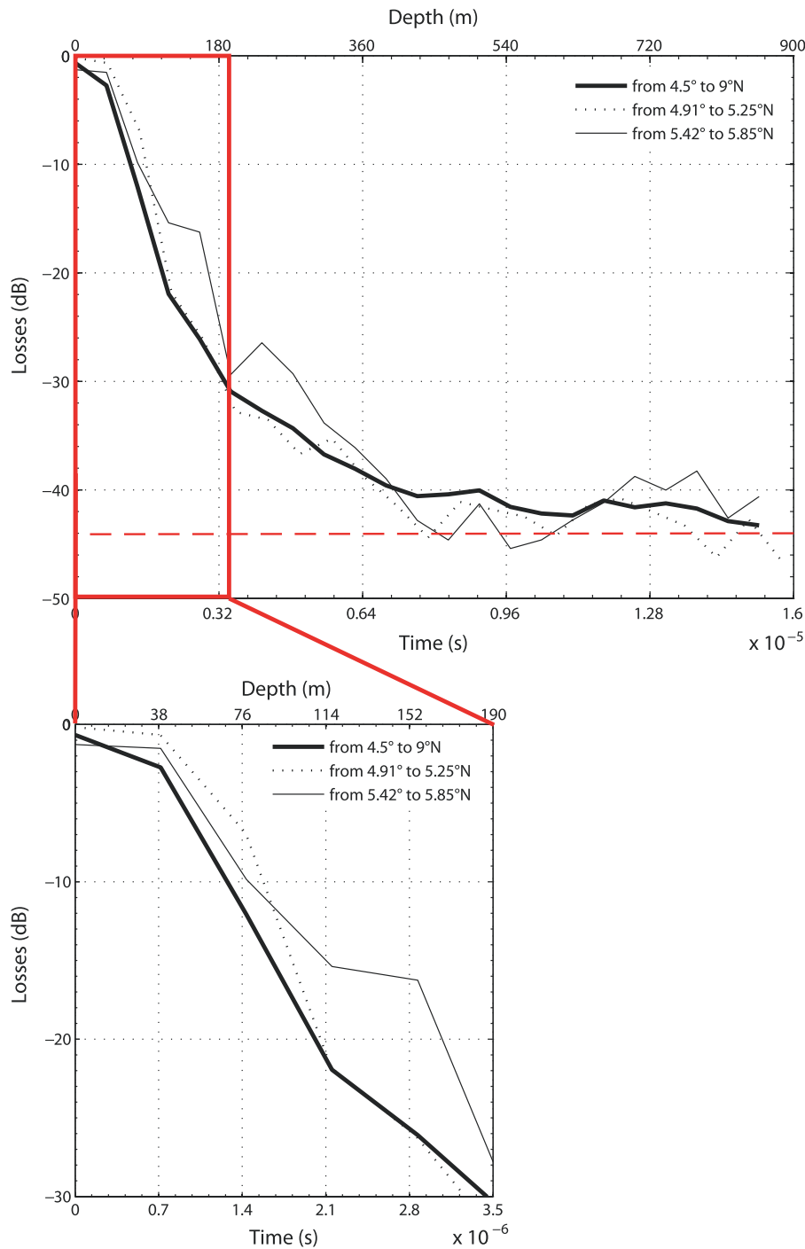
Figure 5. Losses for radar traces between 4.5° and 9°N versus range delay time (s) and depth (m), assuming an average real relative dielectric permittivity of 7.7. The thin black line is the mean of backscattered echoes between 5.42° and 5.85°N, where there is an apparent subsurface signal (see Figure 4). The dotted black line is the mean of backscattered echoes between 4.91° and 5.25°N. The thick black line is the mean of backscattered echoes of the study area between 4.5° and 9°N, omitting the segment from 5.42° to 5.85°N. The dashed red line represents the noise level at -42 dB. The enlargement at the bottom illustrates the loss function in the first 3.5 microseconds (red box).
