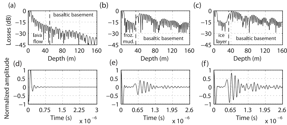
Figure 6. FDTD simulated radar echoes showing (a–c) losses and (d–f) normalized amplitude of the backscattered signal for Model 1 (lava flow model; Figures 6a and 6d), Model 2 (frozen mudflow model, 50% ice/50% basaltic dust; Figures 6b and 6e), and Model 3 (frozen sea model, with a 35-m-thick top layer of ice; Figures 6c and 6f). Black dashed lines represent the interface between the different geoelectrical materials. See Table 1 for material properties. The error on the normalized signal amplitude is 10%.
