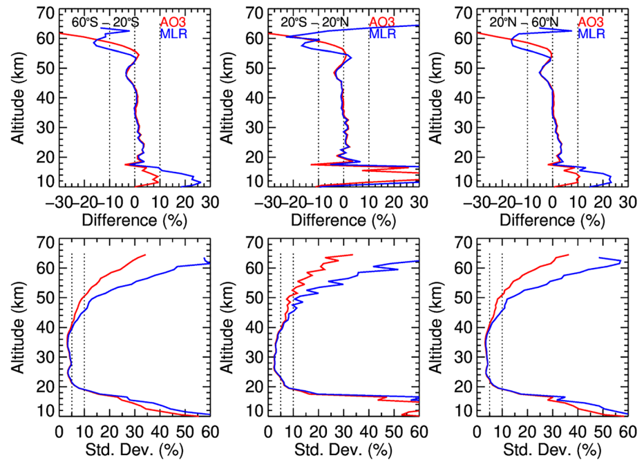
Figure 9. Mean differences (top panel) and standard deviations (bottom panel) between collocated Aura MLS and SAGE III/ISS ozone from AO3 (red) and MLR (blue) retrieval algorithm. Differences and standard deviations are derived in three broad latitude bands, 20°–60°S, 20°S–20°N, 20°–60°N, and represented as a percentage.
