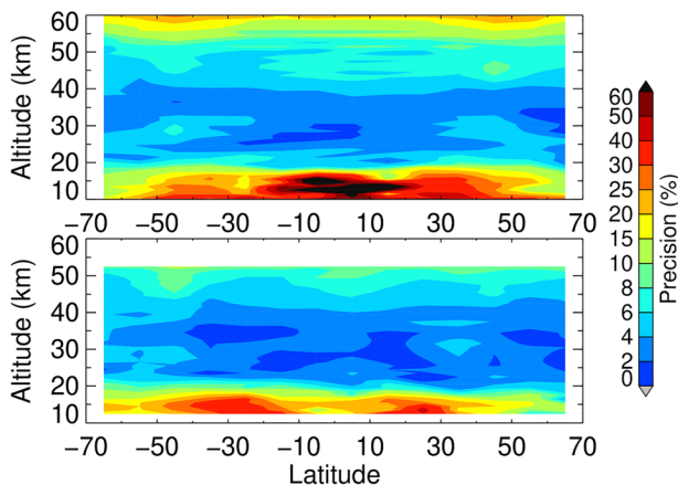
Figure 15. Estimated precision in SAGE III/ISS AO3 ozone based on comparisons with collocated Aura MLS (top) and OMPS LP (bottom) data between June 2017 and May 2019.
