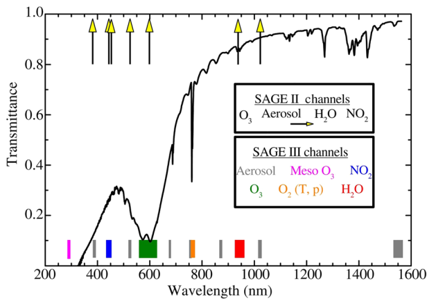
Figure 1. Sample wavelength dependence of atmospheric transmission in the lower stratosphere with locations of the different spectral channels used by the SAGE II (yellow arrows) and SAGE III/ISS instruments (colored boxes). The 12 SAGE III/ISS channels are color-coded by species of interest and are numbered from smallest to largest wavelength.
