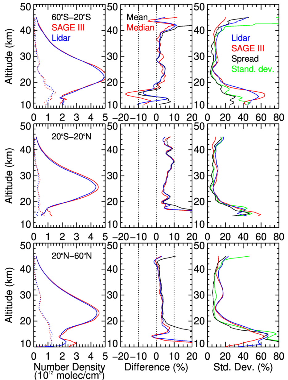
Figure 12. Comparisons between SAGE III/ISS and correlative lidar profiles at three latitude bands, 60°S to 20°S (top panel), 20°S to 20°N (middle panel), and 20°N to 60°N (bottom panel). The mean (solid lines) and standard deviation (dotted lines) of coincident SAGE III/ISS (red) and lidar (blue) ozone number density profiles are shown in the left panel. The relative percentage differences between SAGE III/ISS and lidar are shown in the middle panel. The mean and median relative differences are indicated by the black and red colors, respectively. The blue lines indicates differences estimated from averaged ozone profiles (see text). In the right panel, the standard deviations of mean and 1 - \sigma spreads of median differences are indicated by green and black lines, respectively. The standard deviations of coincident SAGE III/ISS (red) and lidar (blue) profiles are also shown.
