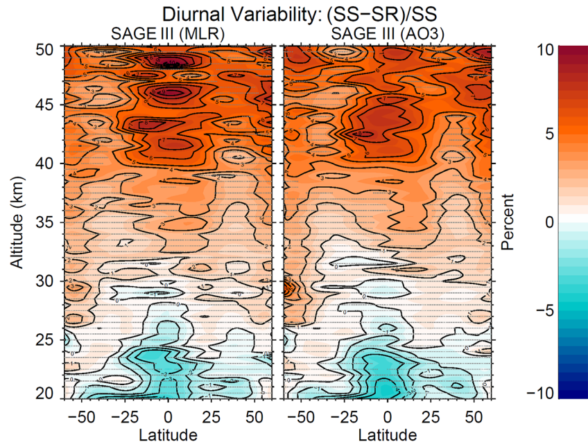
Figure 6. Mean differences between SAGE III/ISS sunrise (SR) and sunset (SS) ozone values from regression model analysis. Results from both MLR (left) and AO3 (right) algorithms are shown. The percentage difference is expressed as (SS-SR)/SS * 100\% . The very fine resolution stippling denotes regions that are not statistically significant at the two-sigma level.
