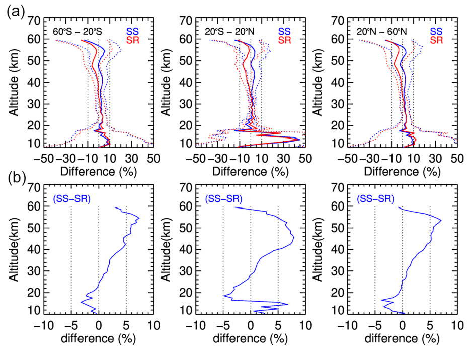
Figure 7. (a) The mean percentage differences (solid line) and standard deviations (dotted line) between SAGE III/ISS AO3 ozone and coincident Aura MLS nighttime measurements between June 2017 and May 2019 in three latitude bands, 60° to 20°S, 20°S to 20°N, and 20° to 60°N. The means and standard deviations of relative differences are separated into SAGE sunrise (red) and sunset (blue) data. (b) The relative differences between SAGE III/ISS sunrise and sunset measurements by using coincident Aura MLS as a transfer standard. The percentage difference is represented as (SS-SR)/MLS * 100.
