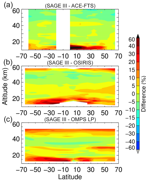
Figure 10. Mean differences between SAGE III/ISS AO 3 ozone and correlative (a) ACE-FTS, (b) OSIRIS, and (c) OMPS LP (bottom panel) measurements. Differences are represented as (SAGE-other)/other * 100%.
