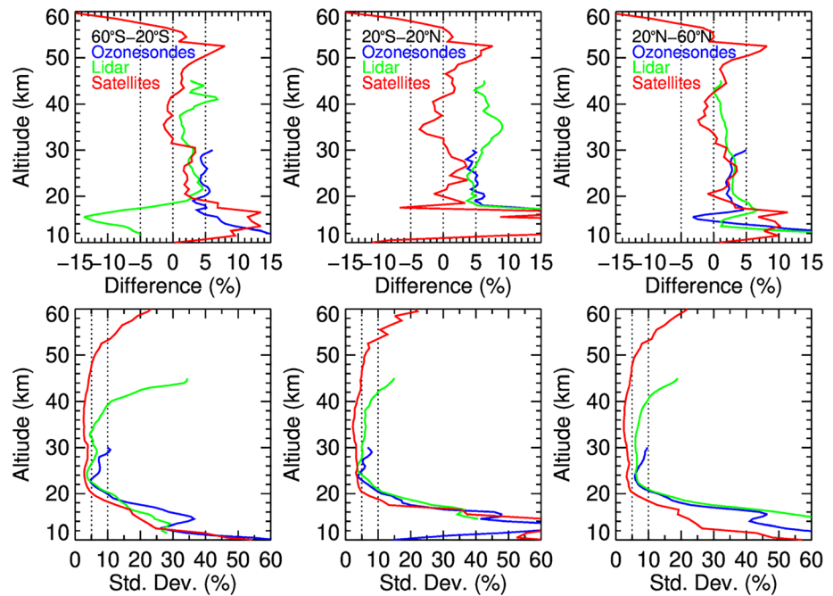
Figure 14. Mean (or median) differences (top panel) and the standard deviations (or spreads) of differences (bottom panel) between SAGE III-ISS ozone and coincident measurements from satellites (red line), lidar (green line), and ozonesondes (blue line) at three latitude bands, 60°S to 20°S (left column), 20°S to 20°N (middle column), and 20°N to 60°N (right column). Results between SAGE III and ground-based measurements (lidar and ozonesondes) are based on medians and spreads, while comparisons between SAGE III and other satellites are based on mean and standard deviation.
