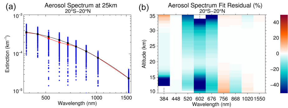
Figure 3. (a) SAGE III/ISS aerosol extinction data from June 2017 to May 2019 at 25 km between 20°S and 20°N at each of the nine aerosol wavelengths (blue dots). The median extinction values at each wavelength are shown by red squares, with the red line being a simple linear interpolation between points to aid the eye in seeing the spectrum. The log of extinction is fit with the log of wavelength using a simple quadratic function for each event at this altitude, and the median of fit values is shown in black. A dip between the data and the fit is clearly visible in the channels surrounding the Chappuis. (b) The median value of the relative residuals between the data and the fit to the aerosol spectrum (i.e., (\text{data}-\text{fit})/\text{fit} ) at each wavelength and altitude for the same latitude range and time period as (a). Results at midlatitudes are similar, simply shifted down in altitude. Gray stippling denotes areas where aerosol extinction data does not exist. The median residuals in the channels used for the quadratic fit are <1% between ~20 and 30 km.
