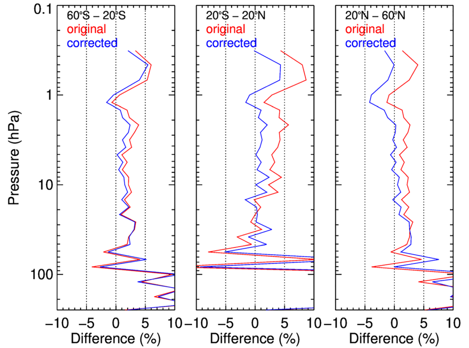
Figure A1. Mean differences between SAGE III/ISS AO3 ozone and collocated Aura MLS data at three latitude bands 60°S to 20°S (left column), 20°S to 20°N (middle column), and 20°N to 60°N (right column). SAGE ozone profiles are converted to MLS coordinates by using reported (red) and bias corrected (blue) temperature and pressure profiles. The percentage difference is calculated as (SAGE-MLS)/MLS * 100%.
