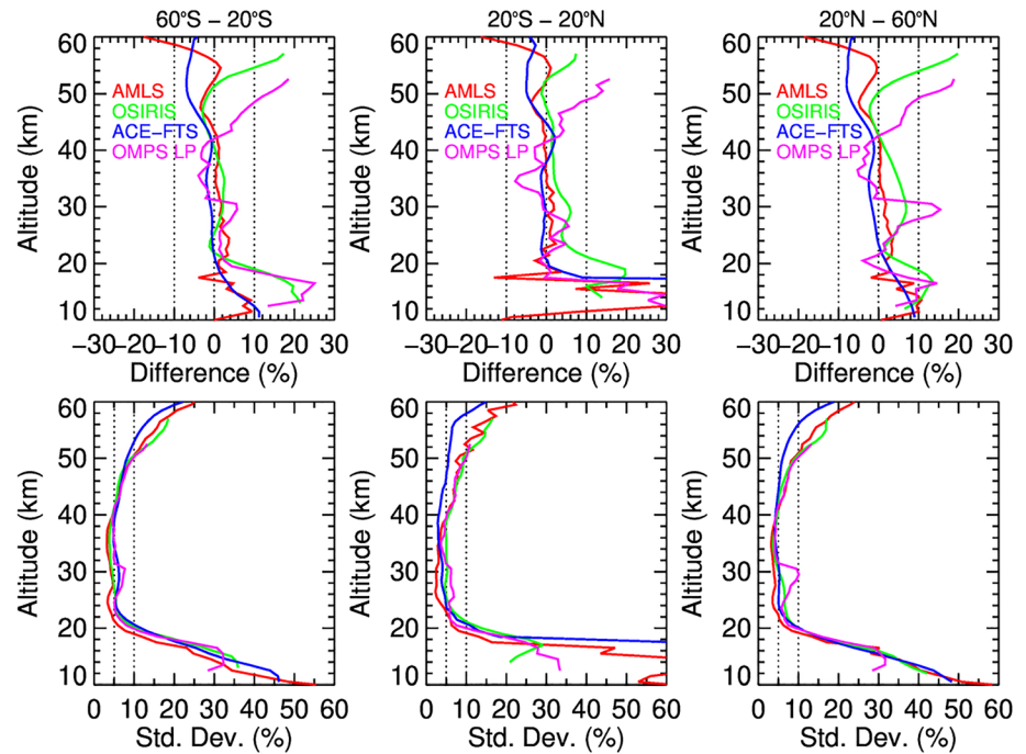
Figure 11. Mean differences (top) and standard deviations (bottom) between SAGE III/ISS AO3 against Aura MLS (red), ACE-FTS (blue), OSIRIS (green), and OMPS LP (pink) in three wide latitude bands.
