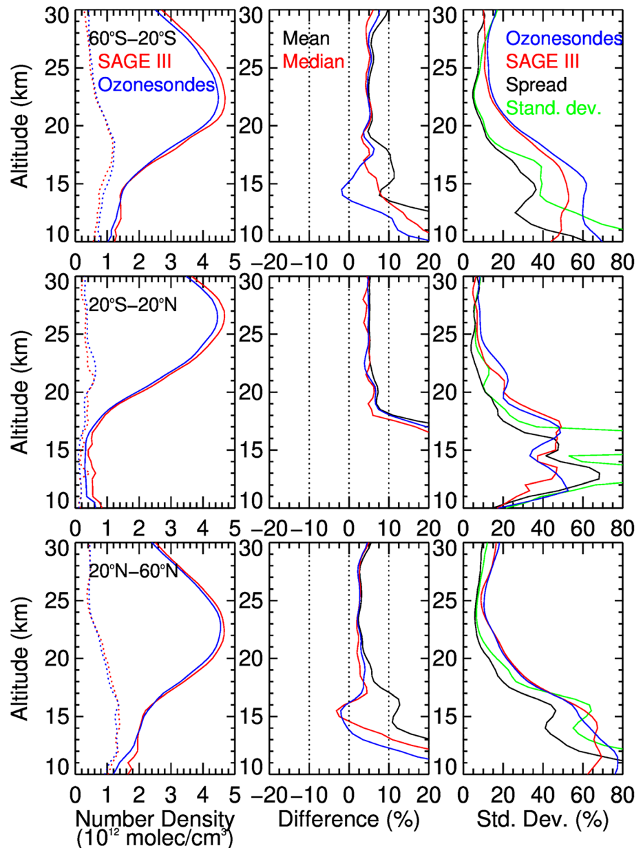
Figure 13. Similar to Figure 12 but for comparisons between SAGE III/ISS and ozonesondes.
