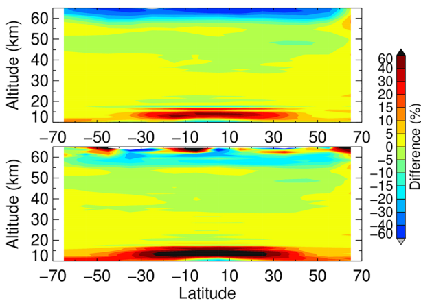
Figure 8. Mean differences between Aura MLS nighttime measurements and ozone retrieved from SAGE III/ISS AO3 (top) and MLR (bottom) algorithm as a function of latitude and altitude. Positive differences (in percentage) indicate the SAGE III/ISS ozone values are higher than Aura MLS.
