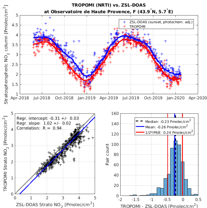
Figure 4. Upper panel: Time series of S5p NRTI stratospheric \text{NO}_2 column data co-located with ground-based SAOZ sunset measurements performed by CNRS/LATMOS at the NDACC mid-latitude station of Observatoire de Haute-Provence (France). The latter were adjusted for the photochemical difference between the S5p and twilight solar local times, while S5p data were averaged over the ground-based twilight air mass. Solid lines represent 2-month running medians. Lower panels: Scatter plot (left-hand side) and histogram of the difference (right-hand side) with several statistical measures of the agreement between data.
