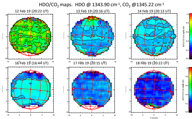
Fig. 9. Maps of the line depth ratio of the weak HDO transition (at 1344.90 cm -1 ) to the CO 2 transition at 1345.22 cm -1 , recorded during the February 2019 run. Data are the same as in Figs. 2 and 5. The sub-solar point is shown as a white dot. Times refer to the mid-times of the observations.
