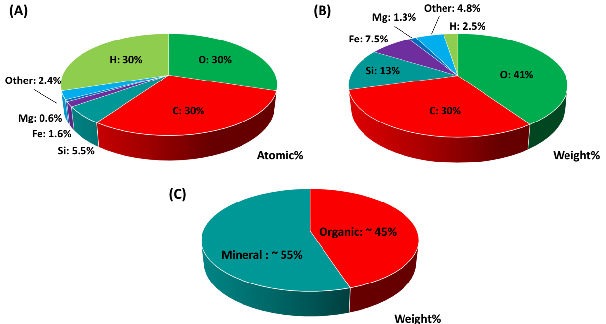
Figure 10. Averaged composition of 67P's dust particles as deduced from COSIMA measurements and some hypotheses detailed in the text. The averaged composition is given (a) by atomic fraction and (b) by atomic mass fraction. Image (c) is the mineral and organic content estimated in mass fraction.
