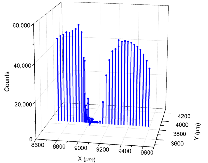
Figure 2. Spatial distribution of the PDMS intensity for the analysis of the particle Kenneth. The counts of the PDMS fragment \text{Si}(\text{CH}_3)_3^+ is displayed on (lowest values) and off (highest values) the particle.
