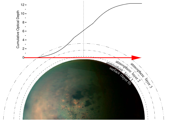
Figure 3. This figure shows a stylized representation of an example photon traverse through Titan's atmosphere. The plot shows the cumulative optical depth as a function of distance along a photon traverse indicated by the red ray. SRTC++ uses this type of cumulative optical depth function within a photon traverse to both calculate net atmospheric opacity and to ascertain the location in physical space at which a scattering event occurs, translating from optical depth space. We do that by generating a random photon optical depth \tau_{\text{random}} at which the next scatter occurs from Equation (1) and then tracing that \tau_{\text{random}} to its corresponding location along the traverse in this plot. This particular photon's photon traverse heads in from deep space, encounters Titan's outer atmosphere, and then continues down before reaching a closest approach in the troposphere and above the surface. It then heads back out into space. The breaks in slope occur at the interfaces between atmospheric layers as specified in the Tomasko et al. (2008) atmospheric model.
