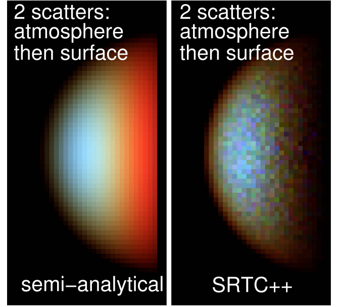
Figure 8. These images show the spatial results from the _{10} calculations described in Section 3 for both the semianalytical model (left, from Equation (9)) and SRTC++ (right). The relatively low S/N evident in the pixel-to-pixel variation results from (1) selecting only that fraction of photons that experience the specific history _{10} (i.e., ones that first bounce off of the atmosphere, then bounce off of the surface and arrive at the detector) and (2) using this many photons allowed us to sufficiently demonstrate that SRTC++ satisfactorily reproduces known plane-parallel results as shown in Figure 7. Running additional photons always improves the S/N, but takes progressively longer owing to the S/N's dependence on the square-root of the number of photons input. The colors map red to 5.0 \mu\text{m} , green to 2.0 \mu\text{m} , and blue to 1.3 \mu\text{m} . This image depicts a uniform sphere of albedo 1.0 illuminated from the left at 90^\circ phase angle. Hence the strong red signal in the semianalytical case comes from geometry near the terminator with high incidence angle i —a regime in which its plane-parallel assumptions break down.
