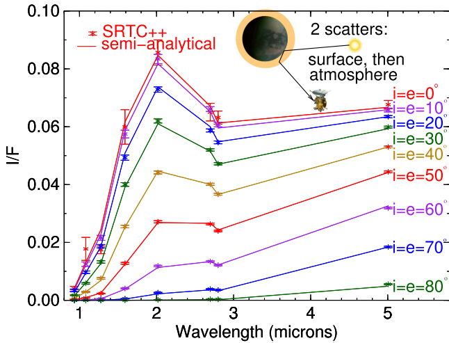
Figure 9. This figure represents our last comparison between SRTC++ and the semianalytical model. In this two-scatter, surface-then-atmosphere case, the lines show Equation (10) and the asterisks with error bars show the SRTC++ result. Although the semianalytical values match those from the atmosphere-then-surface case (Figure 7), the higher SRTC++ noise here (i.e., lower S/N) results from Titan’s highly forward-scattering haze particles’ phase function (see the text).
