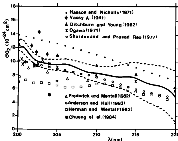
Fig. 3 The O 2 absorption cross-sections as a function of the wavelength from 200 to 220 nm. The solid line joins the values of \sigma_{iO_2} averaged over 10 steps of the scan. The dashed lines show the minimum and maximum possible values of \sigma_{iO_2} averaged over 10 steps of the scan due to the systematic errors in the ozone column content and in the calibration in wavelength. Earlier measurements are indicated with different symbols.
