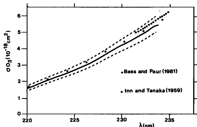
Fig. 2 The O 3 absorption cross-sections as a function of the wavelength from 220 to 235 nm. The solid line joins the values of \sigma_{iO_3} averaged over 10 steps of the scan. The dashed lines show the minimum and maximum possible averaged values due to the systematic errors in the ozone column content and in the calibration in wavelength.
