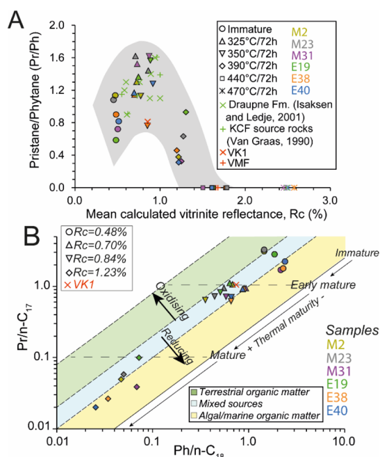
Figure 7. (A) Plot of pristanes/phytane vs the mean calculated vitrinite reflectance and (B) evolution of Pr/ n -C 17 versus Ph/ n -C 18 ratios (from Shanmugam 58 ) for artificially matured KCF samples and naturally matured rocks from the Viking graben (VK1) and the Vaca Muerta fm. (VMF). (A) Comparison with pristanes/phytane of natural rocks from the Draupne (Isaksen and Ledje 59 ) and the KCF (van Graas 60 ). The highly oil-prone samples are M31, E38, and E40.
