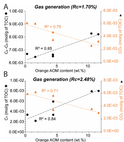
Figure 9. Evolution of (A) C 2 –C 5 and (B) C 1 concentrations in Kimmeridge clay samples with increasing initial orange AOM content.
