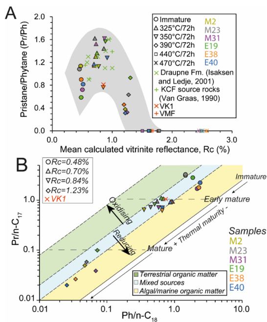
Figure 7. (A) Plot of pristane/phytane vs the mean calculated vitrinite reflectance and (B) evolution of Pr/n-C_{17} versus Ph/n-C_{18} ratios (from Shanmugam 58 ) for artificially matured KCF samples and naturally matured rocks from the Viking graben (VK1) and the Vaca Muerta fm. (VMF). (A) Comparison with pristane/phytane of natural rocks from the Draupne (Isaksen and Ledje 59 ) and the KCF (van Graas 60 ). The highly oil-prone samples are M31, E38, and E40.
