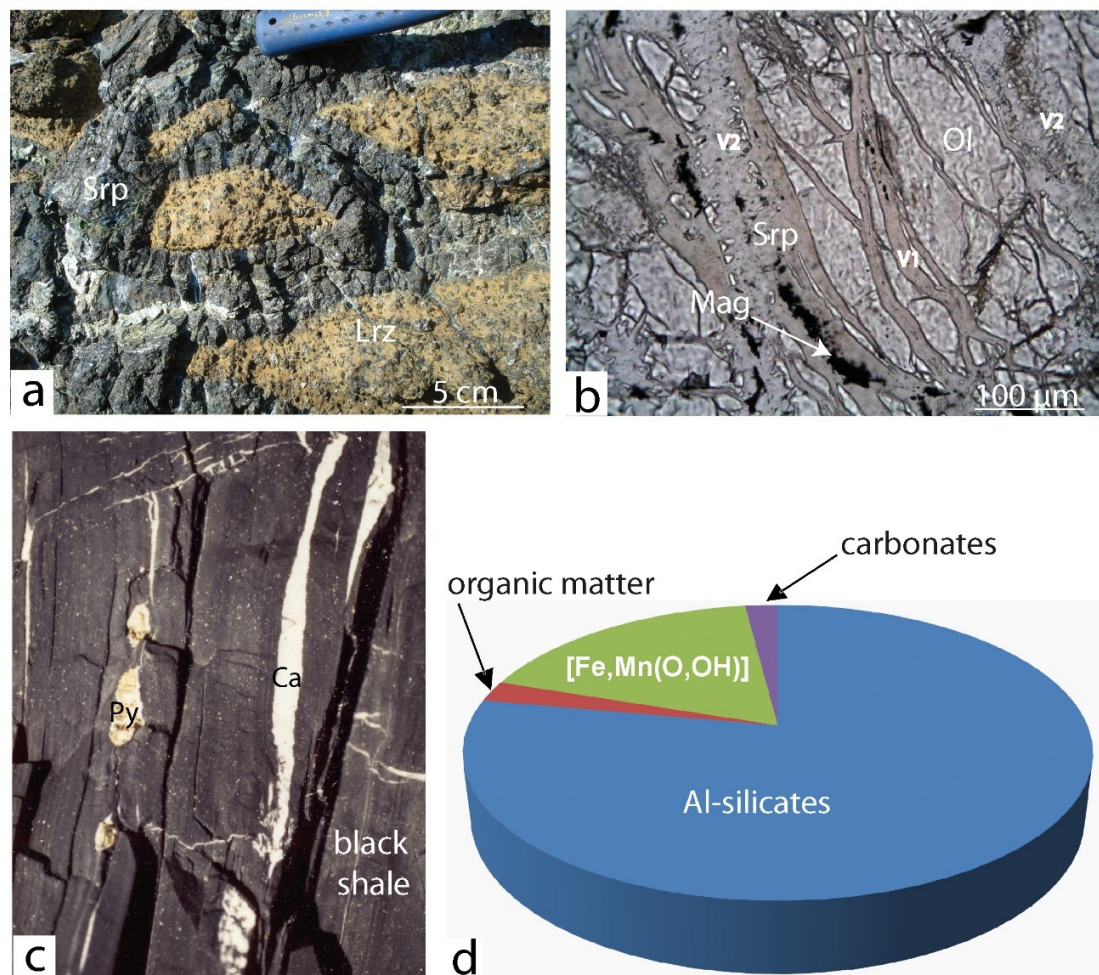
Figure 9. Potential geological sources of chromium (Cr) and vanadium (V) necessary for emerald formation in mafic-ultramafic rocks and black shales: (a) A lizardite (Lrz) that is transformed into serpentinite (Srp), region of Montemaggiore on the Corsican cape, France; (b) Photomicrograph (plane polarized light) of an antigorite vein (V2) cross cutting lizardite veins (V1) and olivine (Ol). Fine-grained magnetite (Mag) is present in the centre of V1; V2 boundaries contain minute secondary olivine grains. Photo: B. Debret; (c) Colombian black shale crosscut by pyrite (Py) -bearing calcite (Ca) veinlets from the Coscuez mine. Photograph: G. Giuliani; (d) Pie diagram representation of the concentration (in %) and relative distribution of beryllium (Be) between the different phases extracted from a black shale containing 4 ppm of ^9\text{Be} , Coscuez mine [54]. OM: Organic matter; [Fe,Mn(O,OH)] = oxy-hydroxides of iron and manganese.
