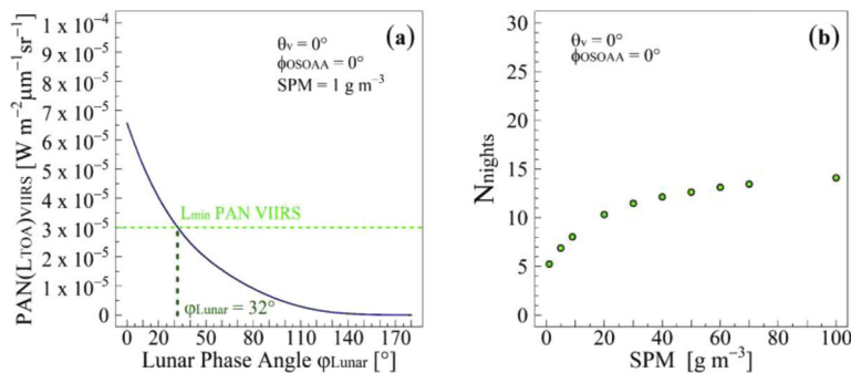
Fig. 10. (a) Relationship between the top of atmosphere radiance \text{PAN}(\text{LTOA}) and the lunar phase angle \varphi_{\text{Lunar}} for a value of \text{SPM} of 1 \text{ g m}^{-3} in the specular plane ( \varphi_{\text{OSOAA}}=0^\circ and \theta_v=0^\circ ), (b) variation of the total number of nights N_{\text{nights}} for which the amplitude of the moon light illumination is sufficiently high to observe SPM as a function of the turbidity.
