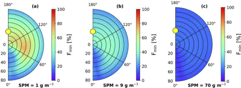
Fig. 9. Spatial variation of the fraction F_{\min} over the observation geometries for various oceanic turbidities: (a) \text{SPM}=1 \text{ g m}^{-3} , (b) \text{SPM}=9 \text{ g m}^{-3} , (c) \text{SPM}=70 \text{ g m}^{-3} . F_{\min} is the minimum value of F from which \text{PAN}(\text{LTOA}) is higher than L_{\min\_PAN\_VIIRS} .
