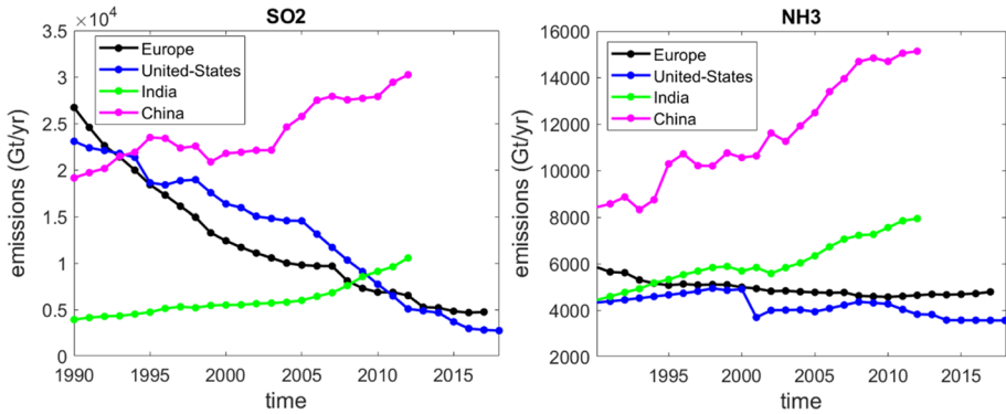
Fig. 2 Trends of emissions of \text{SO}_2 (left panel) and \text{NH}_3 (right panel) over Europe a (black), USA b (blue), India c (green), and China c (magenta). Sources a European Environment Agency (EEA) (2018), b United States Environmental Protection Agency (EPA), c Crippa et al. (2018)
